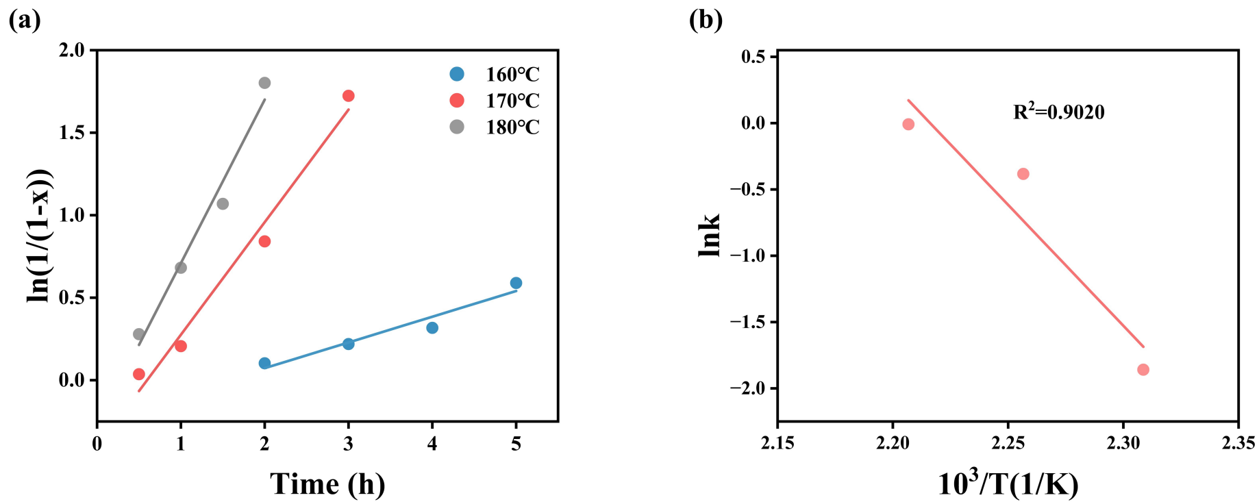
Figure. S11. (a) First-order kinetics at different temperatures; (b) Arrhenius diagram of the rate constant for PET methanolysis.
