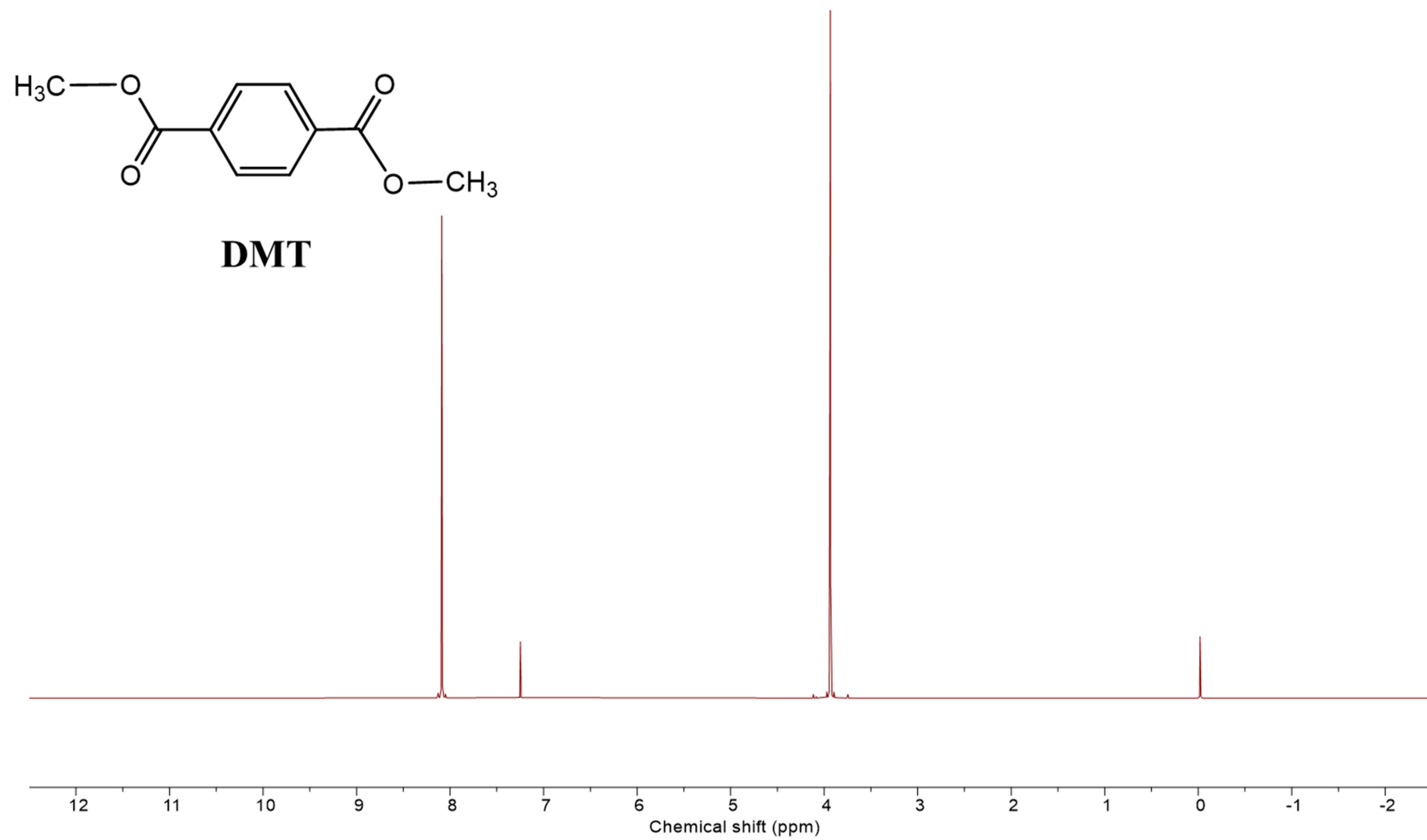
Figure. S12. 1 H NMR spectrum of pure DMT.
