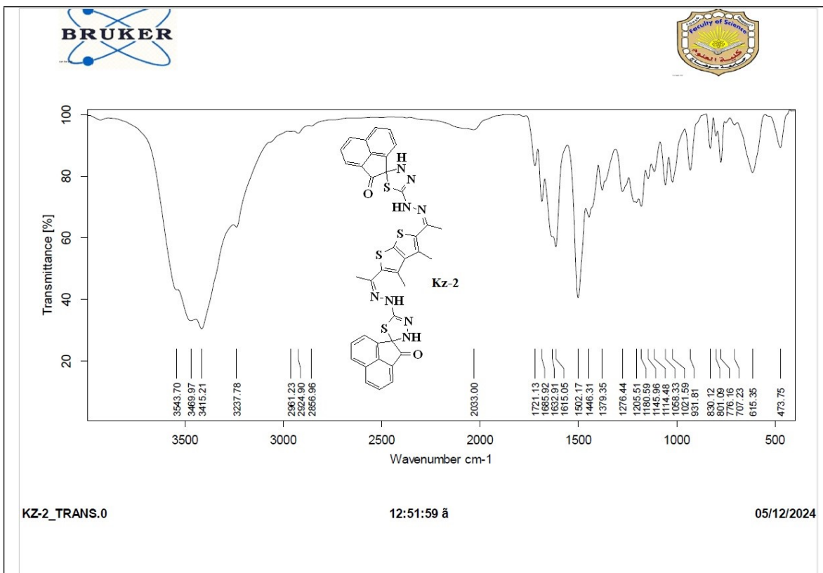
Fig 4: IR Spectrum of compound Kz2
