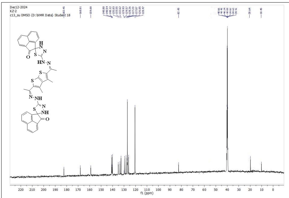
Fig 6: ^{13}\text{C} NMR Spectrum of compound Kz2
