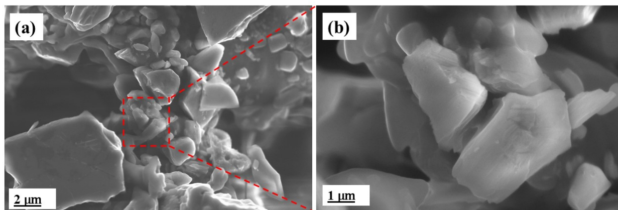
Figure SI 1. (a) SEM micrograph of MAX Phase (b) Magnified image of MAX Phase.
