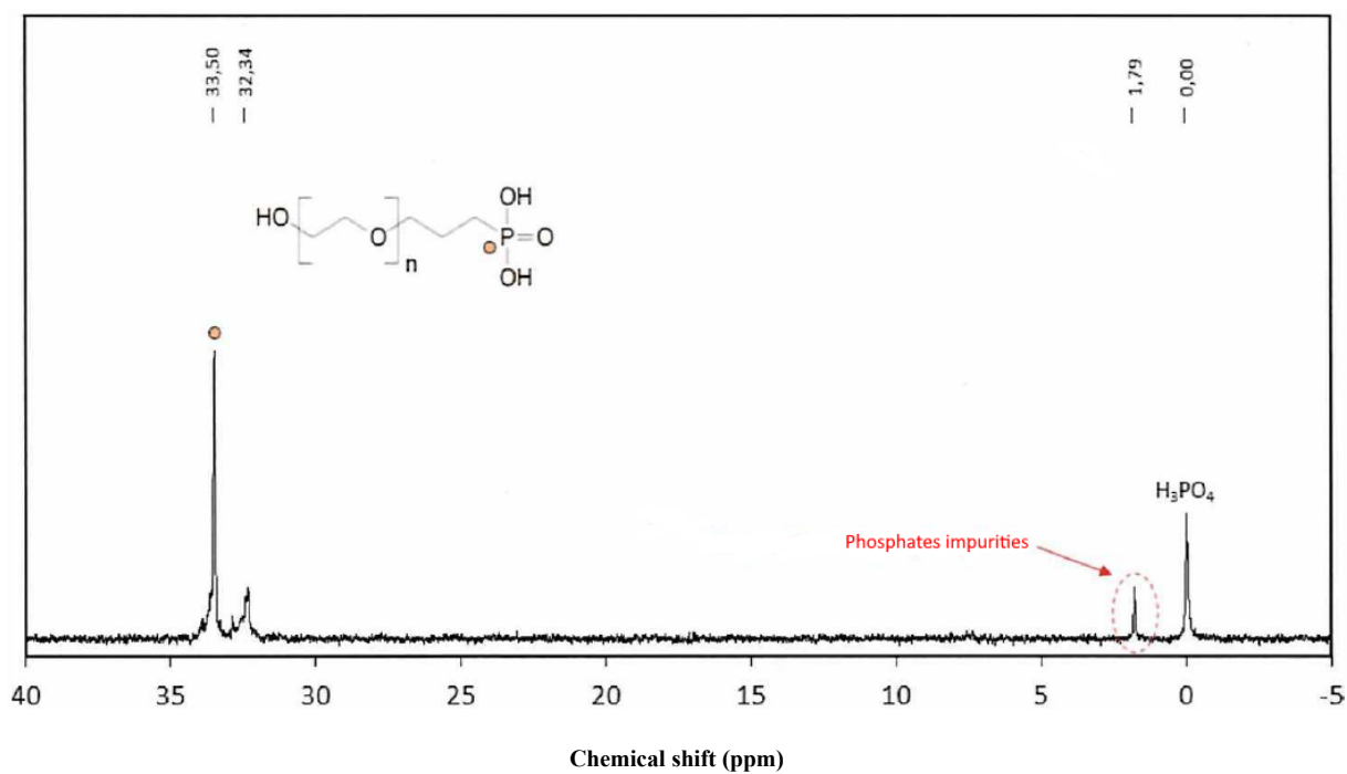
Figure S2 : ^{31}P liquid NMR spectrum of commercial PPEG-10 ligand
