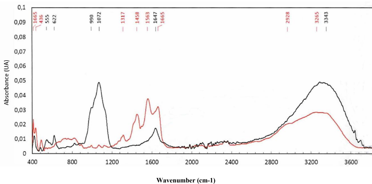
Figure S1 : FTIR spectra of GdF 3 nanoparticles (NPs) before (red line) and after (black line) precipitation in a 5% w/w Na 2 HPO 4 solution.
