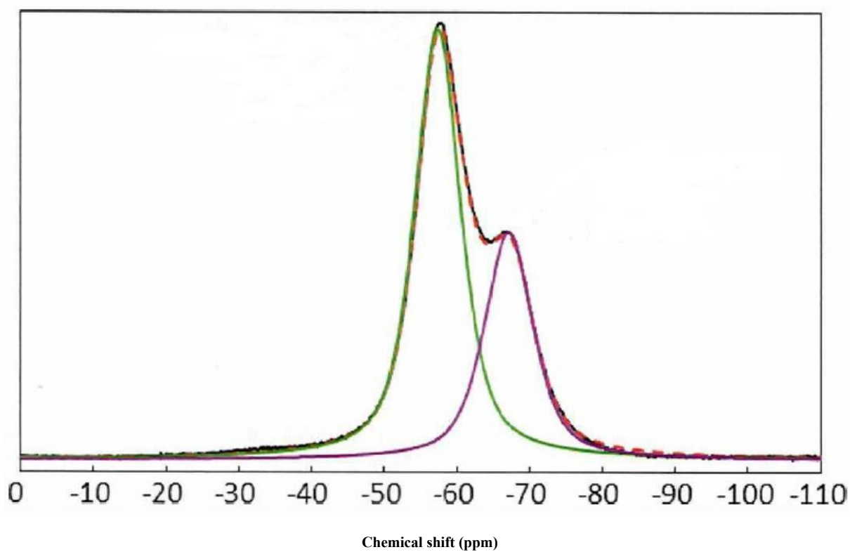
Figure S3 : ^{19}F MAS NMR spectrum of YF3@PPEGi0 nanoparticles after precipitation in 5% w/w Na_2HPO_4 solution.
