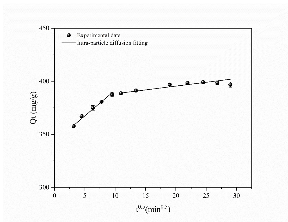
Fig. S1 intraparticle diffusion model for Cr(VI) adsorption
