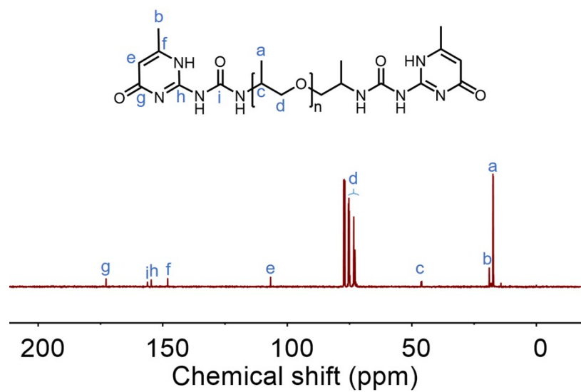
Fig. S7 13 C NMR spectra of USSP 2000 in CDCl 3 (500 MHz, CDCl 3 , 0.1 mg/ml).
