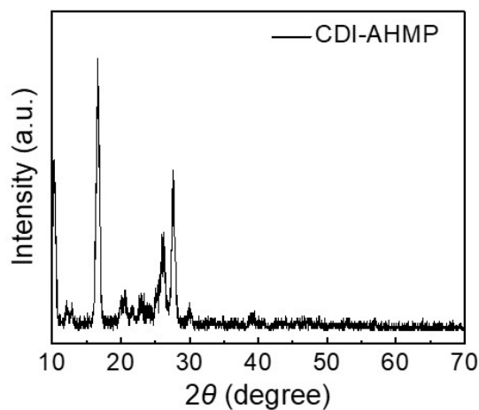
Fig. S1 PXRD patterns of the CDI-AHMP.
