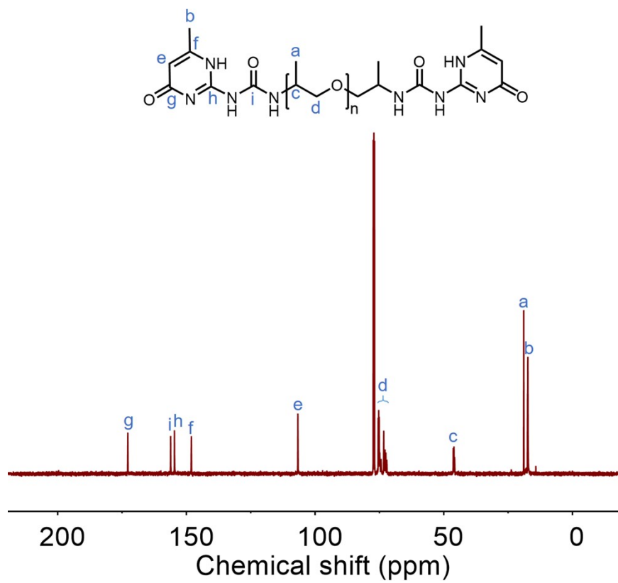
Fig. S6 13 C NMR spectra of USSP 230 in CDCl 3 (500 MHz, CDCl 3 , 0.1 mg/ml).
