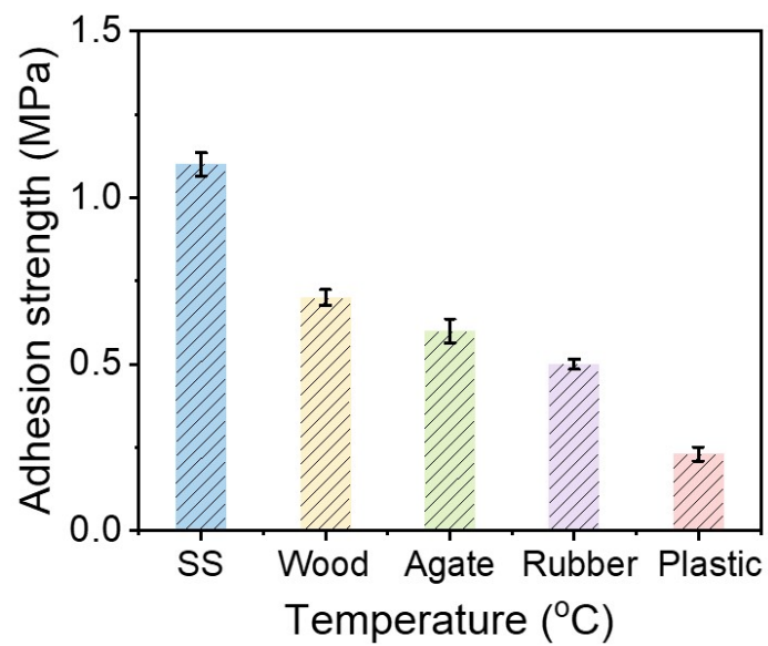
Fig. S10 Adhesion strength of USSP 400 adhesive on various substrates.
