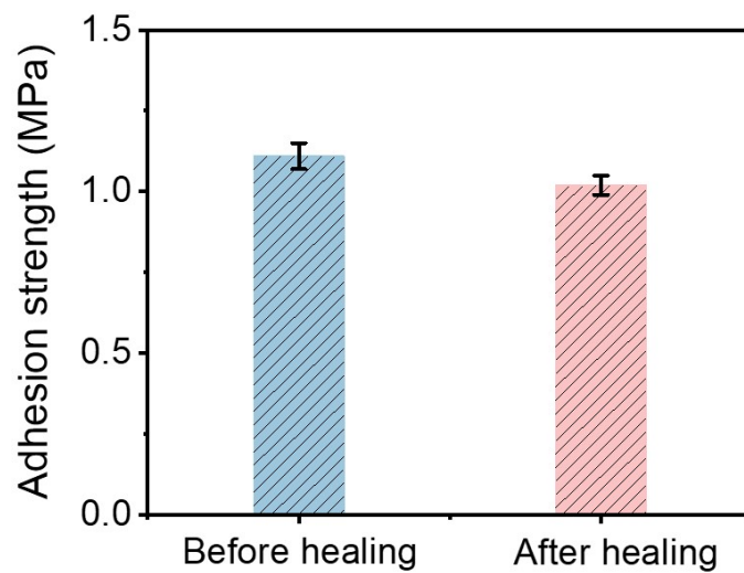
Fig. S9 Adhesion strength of USSP 400 adhesive on SS substrates before and after healing.
