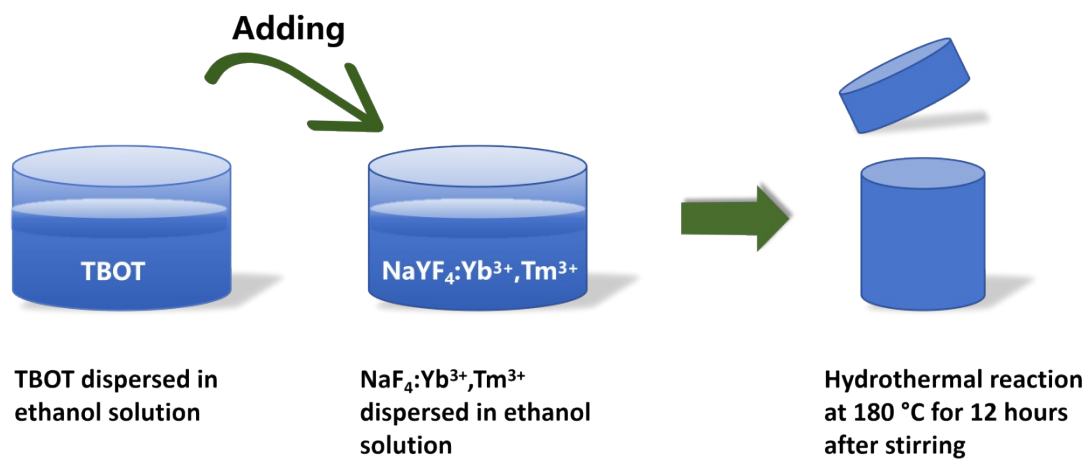
Figure Schematic synthesis route of the as-prepared NaYF 4 :Yb 3+ ,Tm 3+ @TiO 2 microrod composite photocatalysts
