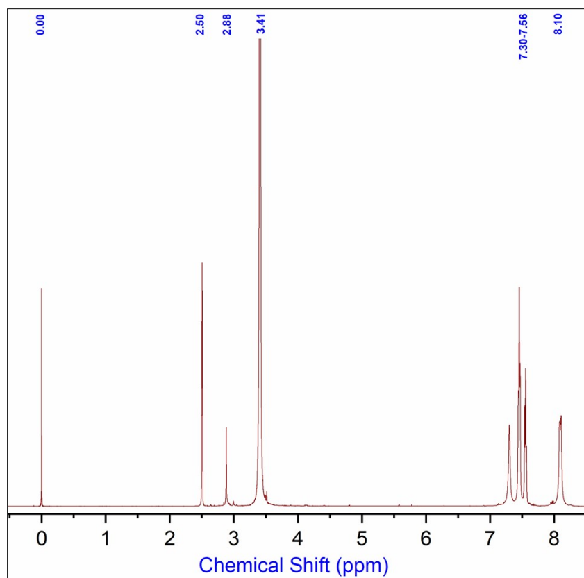
Fig. S6 Proton NMR spectra of SmD
