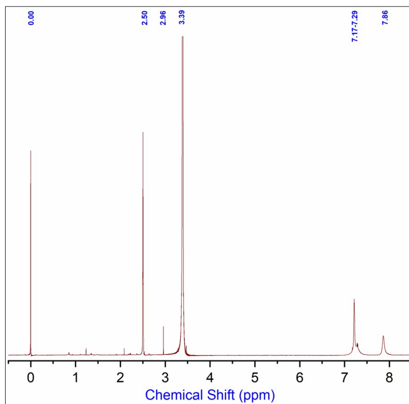
Fig. S4 Proton NMR spectra of SmA
