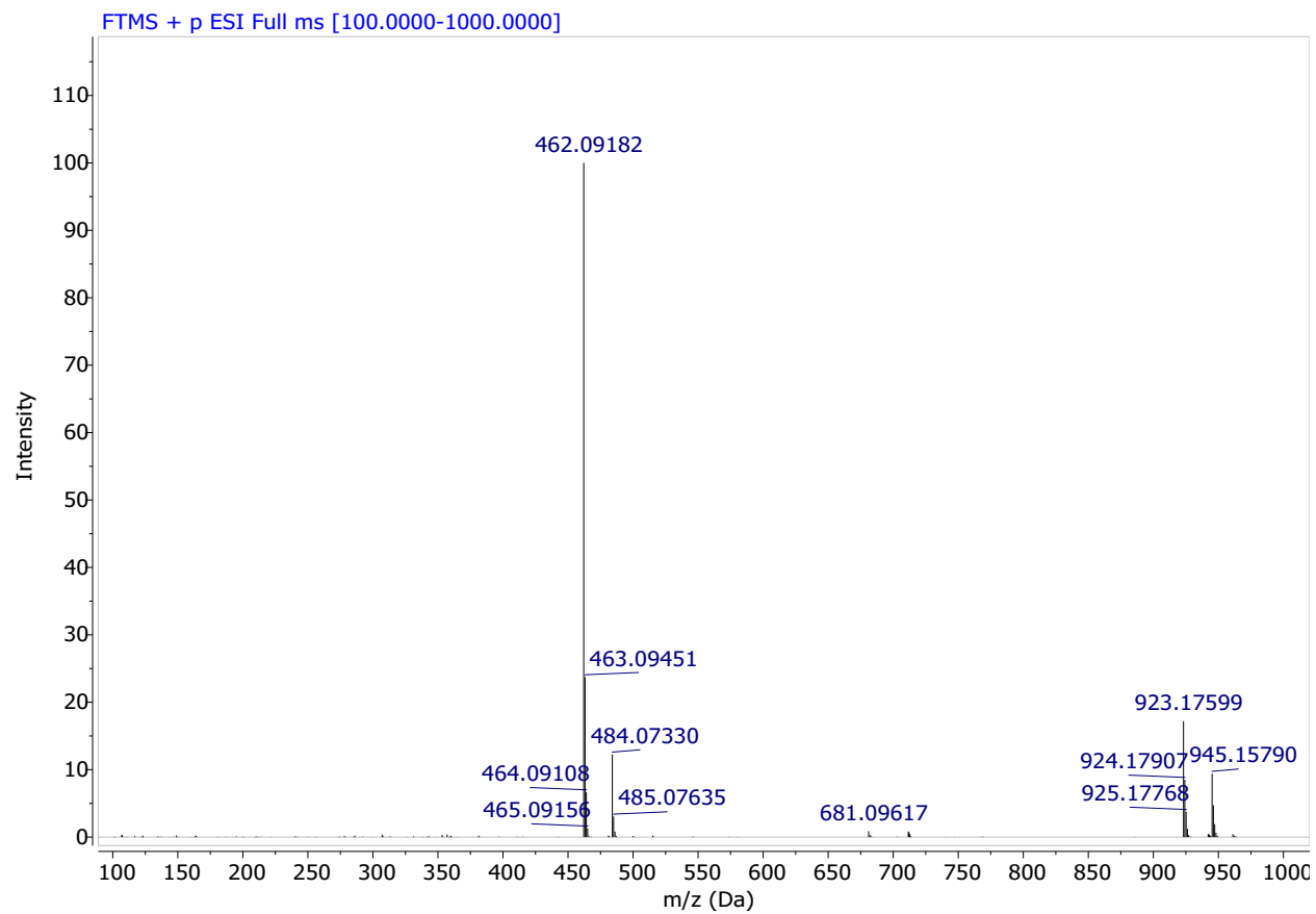
HRMS Spectrum of Compound 5h
