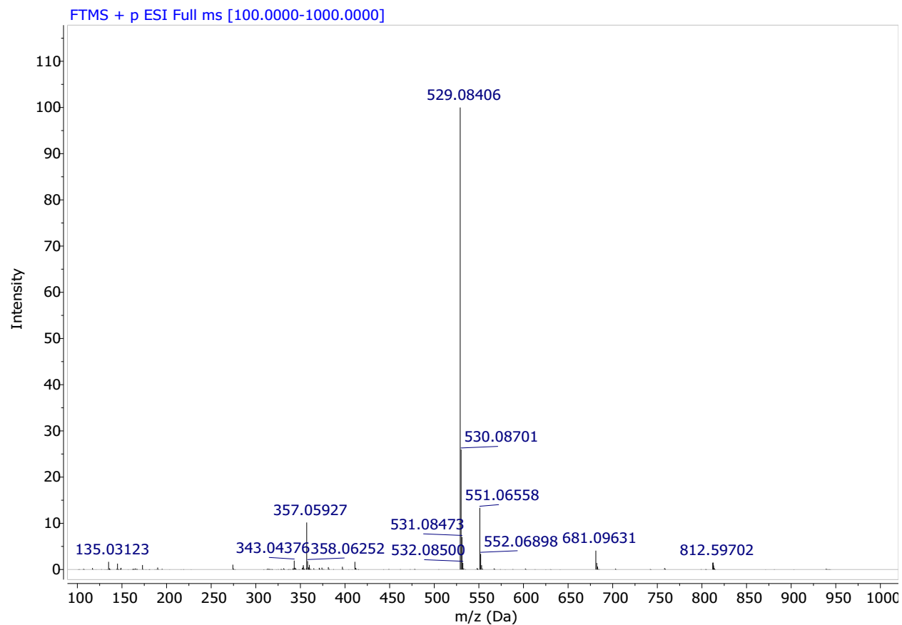
HRMS Spectrum of Compound 5i
