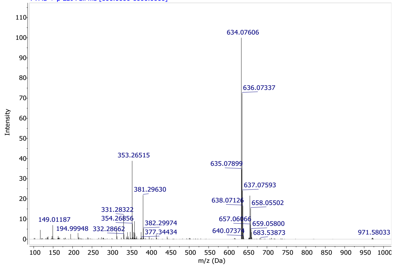
HRMS Spectrum of Compound 5p
