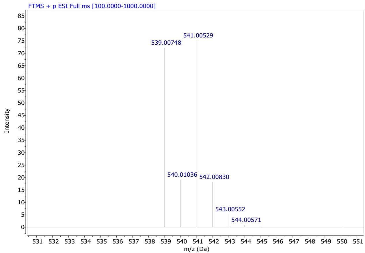
HRMS Spectrum of Compound 5c (Extended)
