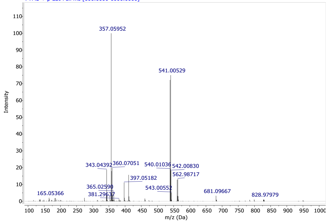
HRMS Spectrum of Compound 5c
