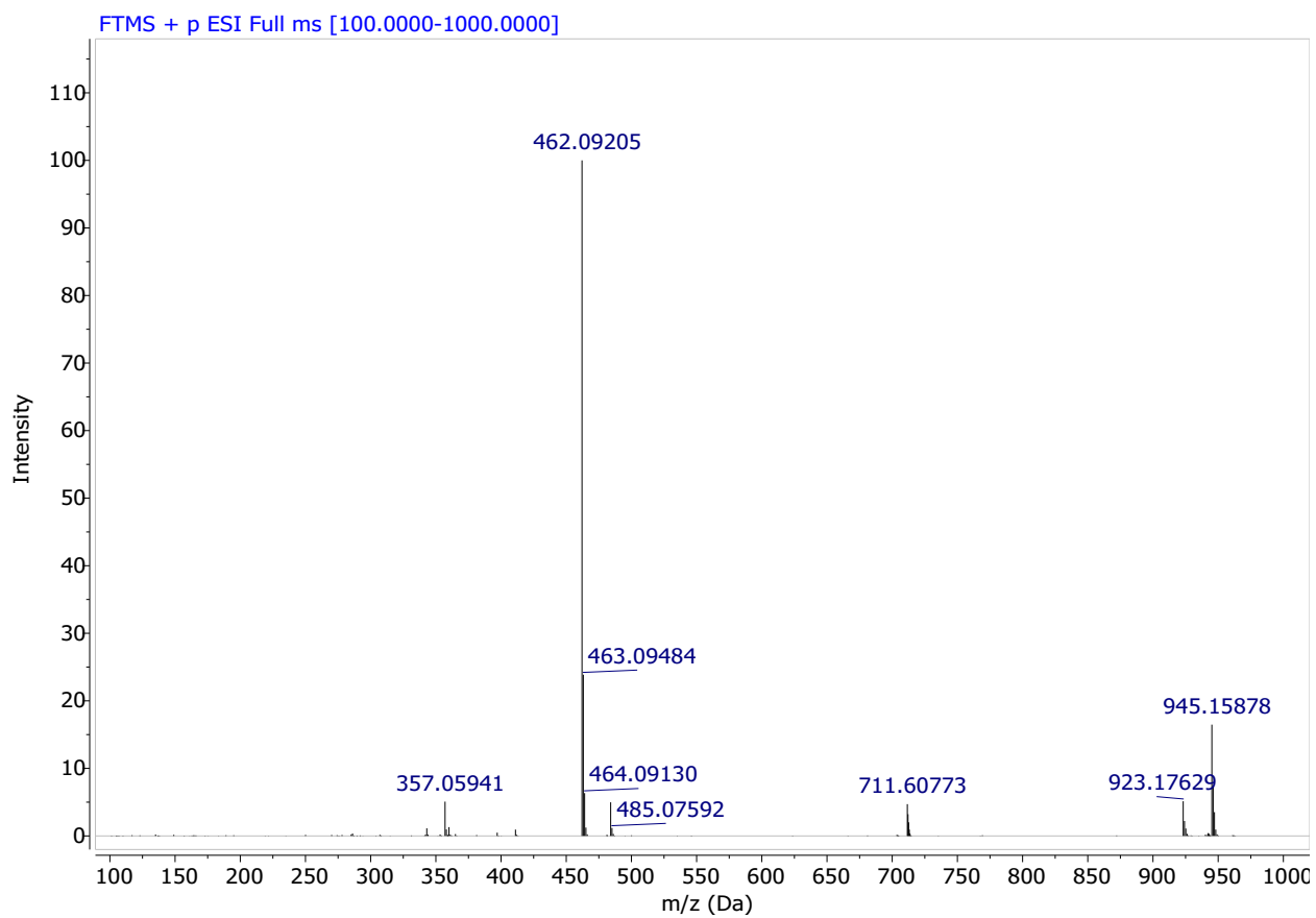
HRMS Spectrum of Compound 5b
