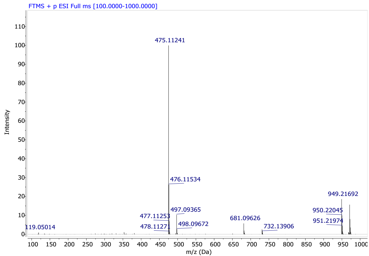
HRMS Spectrum of Compound 5j
