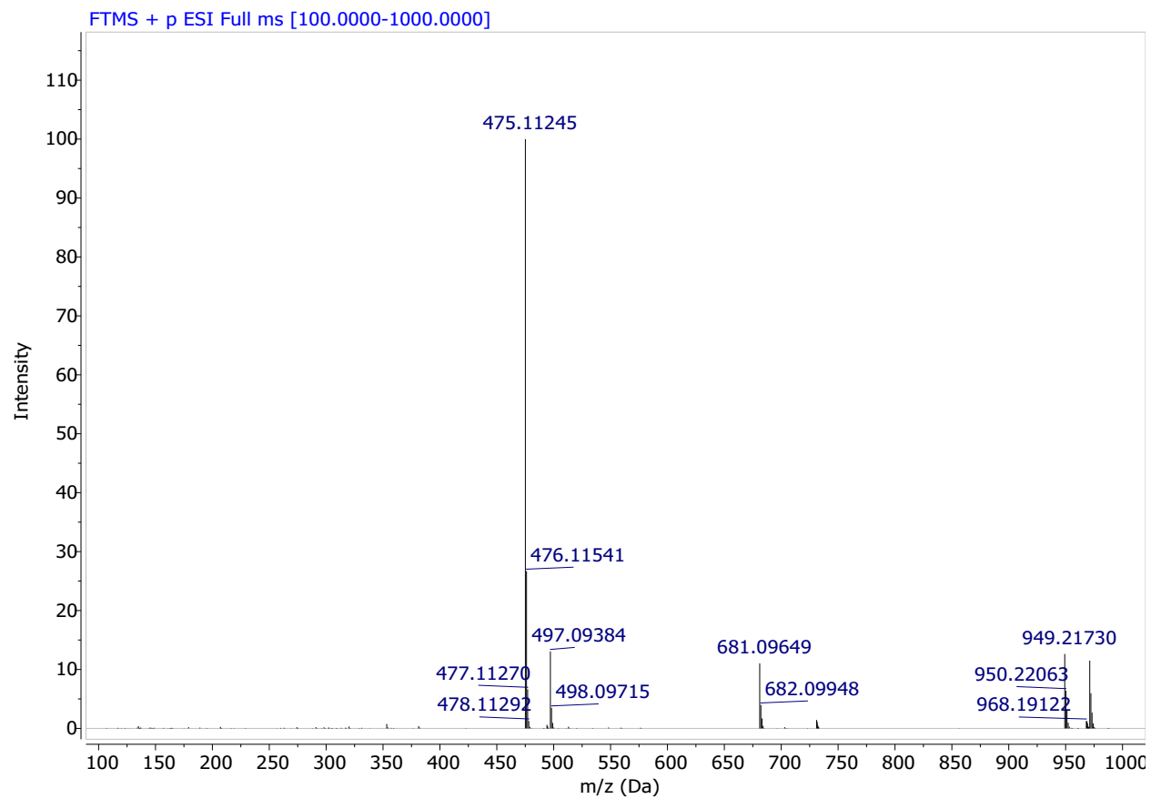
HRMS Spectrum of Compound 5n
