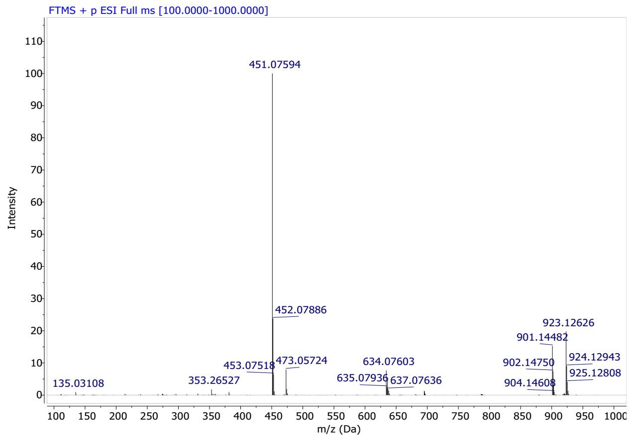
HRMS Spectrum of Compound 5m
