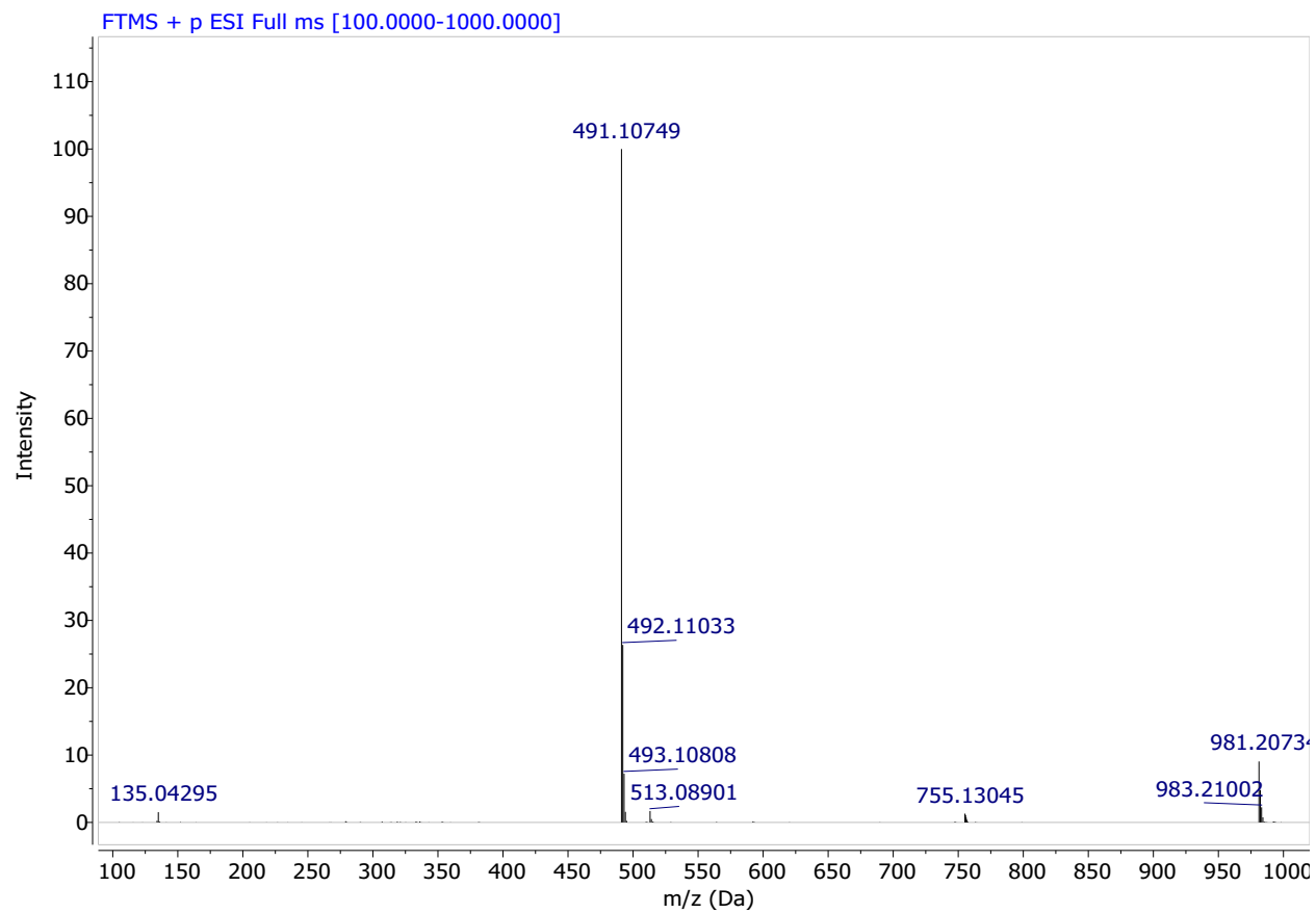
HRMS Spectrum of Compound 5e
