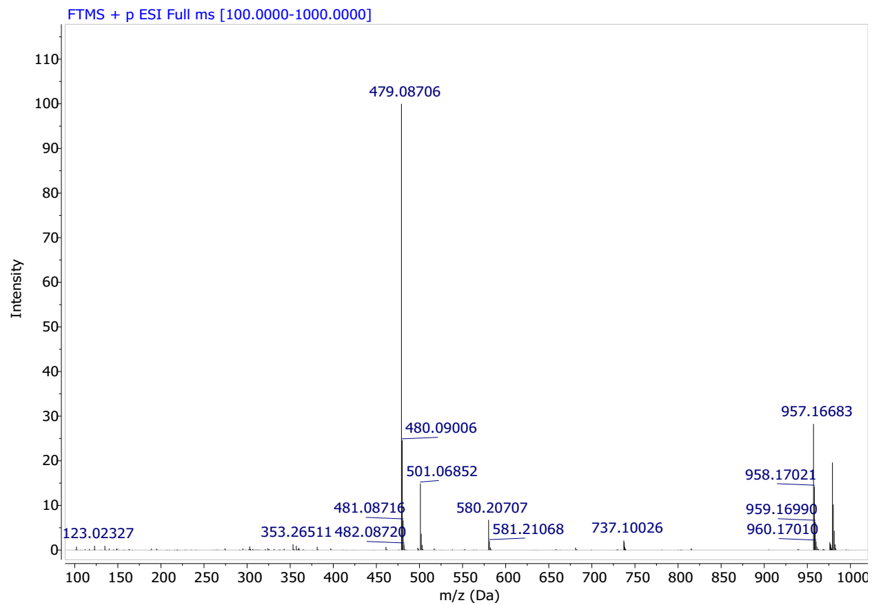
HRMS Spectrum of Compound 5a
