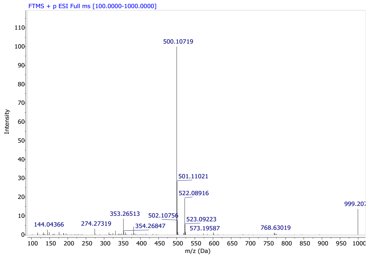
HRMS Spectrum of Compound 5k
