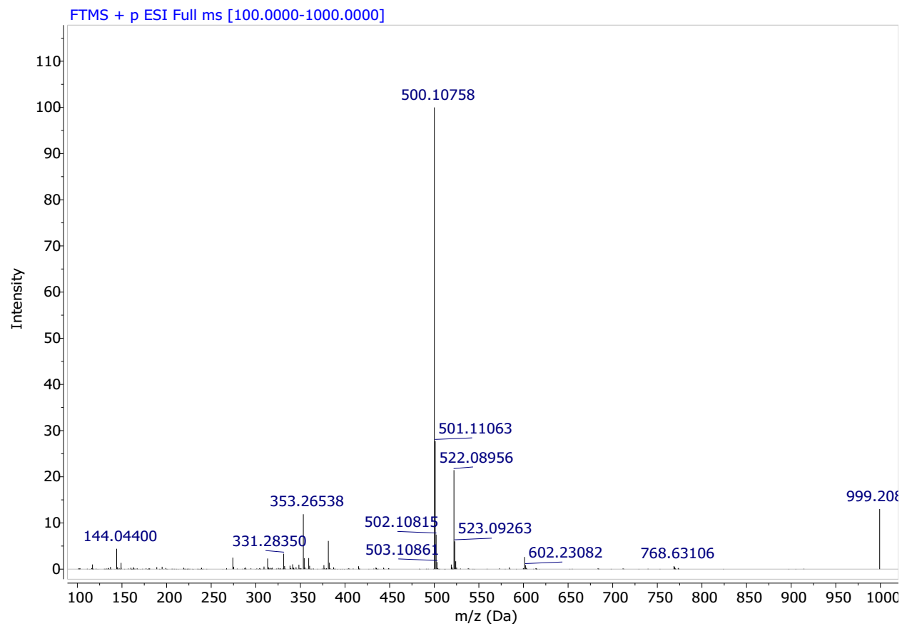
HRMS Spectrum of Compound 5l
