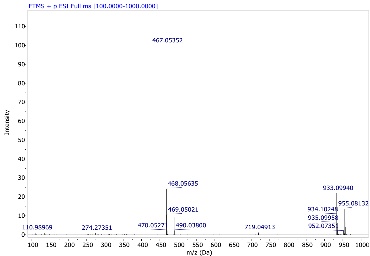
HRMS Spectrum of Compound 5d
