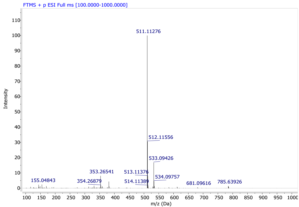
HRMS Spectrum of Compound 5g
