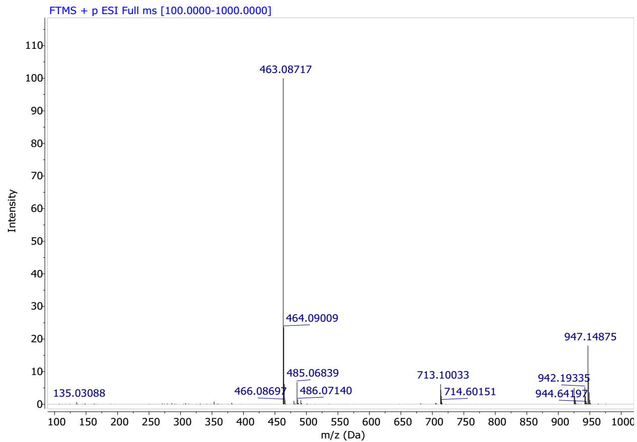
HRMS Spectrum of Compound 5f
