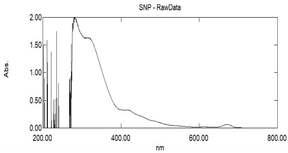
Supplementary Figure 3: UV-Visible graph of Matricaria chamomilla ethanolic extract.
