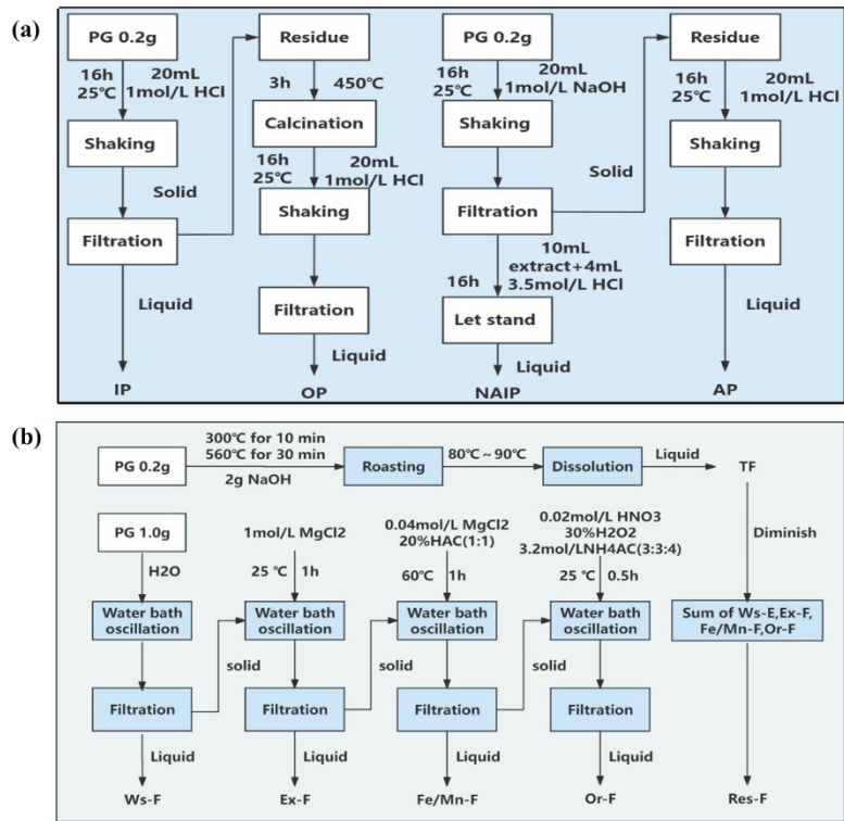
Fig.S1 Sequential extraction procedure for (a) phosphorus speciation analysis and (b) fluorine speciation analysis
