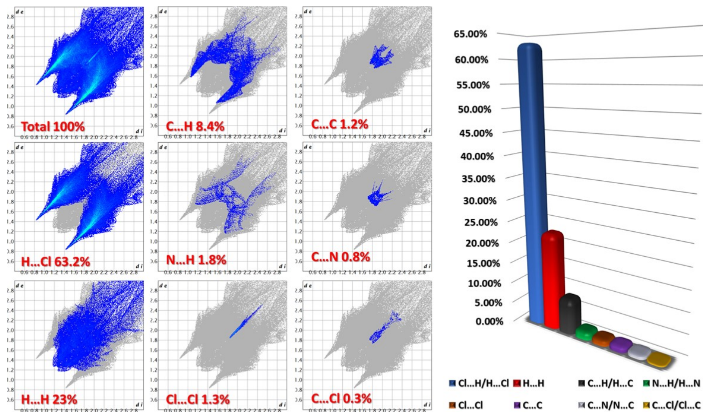
Fig. 3.S: Hydrogen bonding of the titled compound
