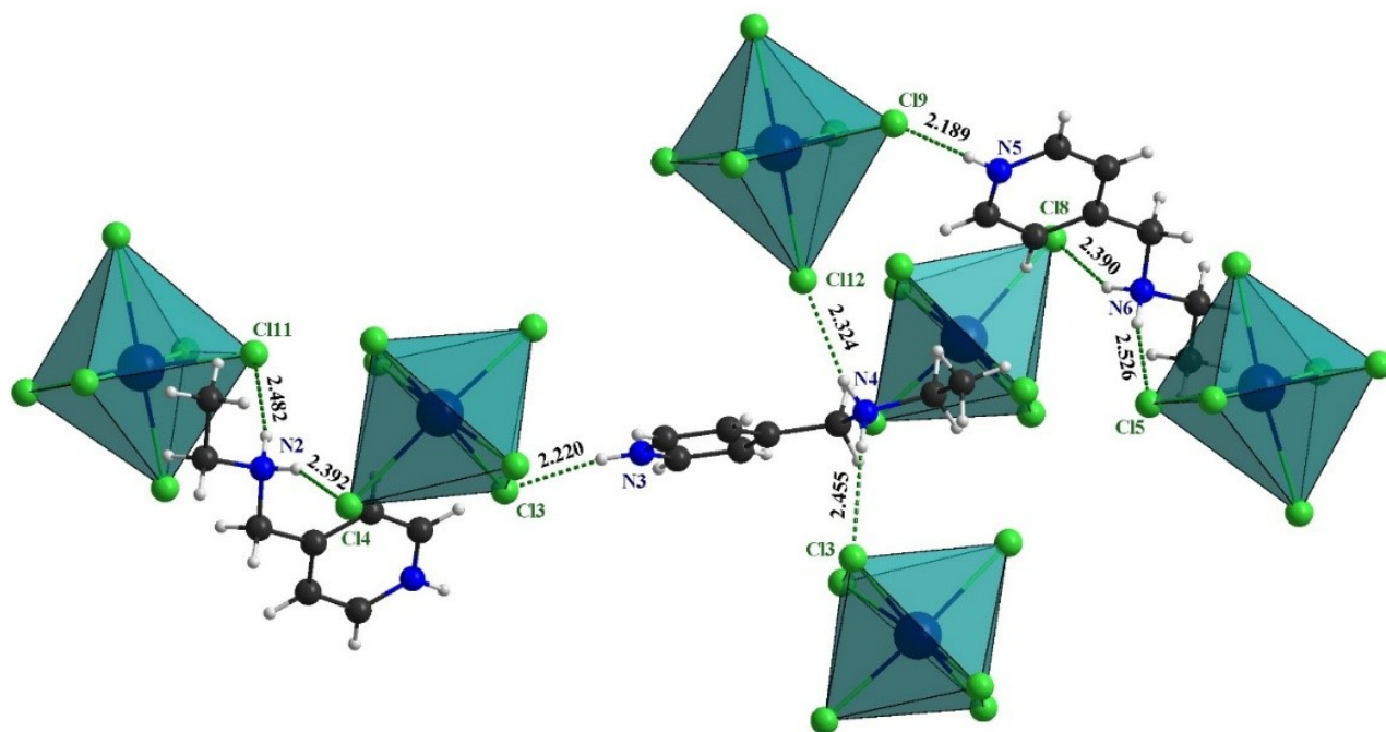
Fig. 3.S: Hydrogen bonding of the titled compound
