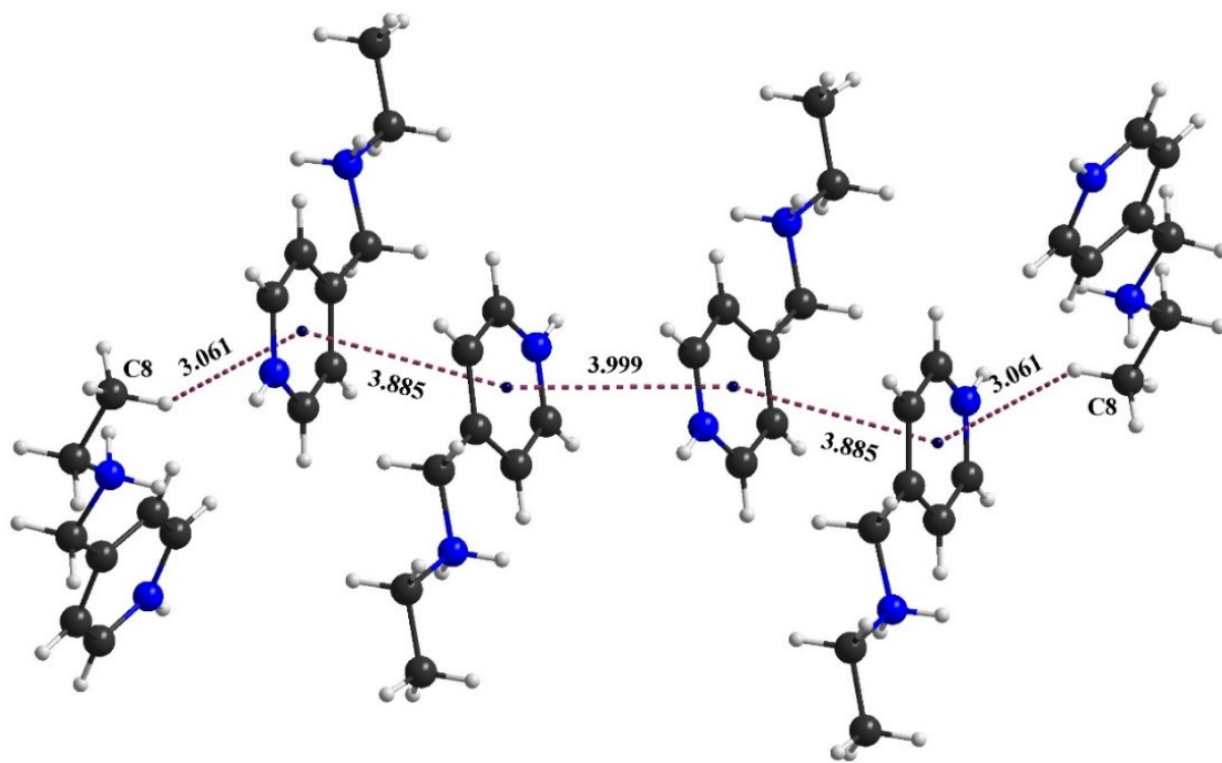
Fig. 2.S: \pi \dots \pi interactions
