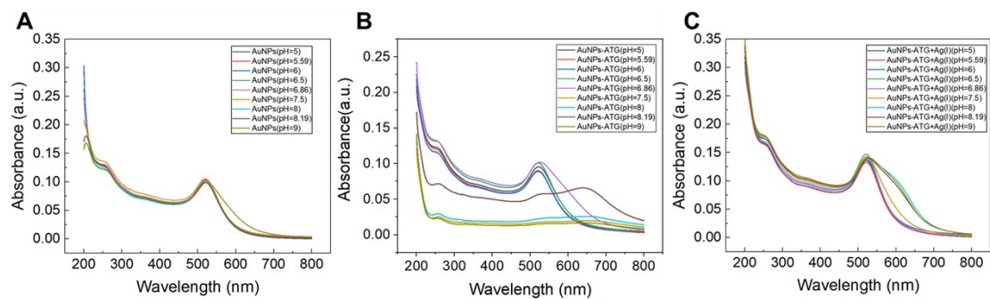
Figure S1. Effect of pH on (A) AuNPs, (B) AuNPs-ATG, and (C) AuNPs-ATG+Ag(I).
