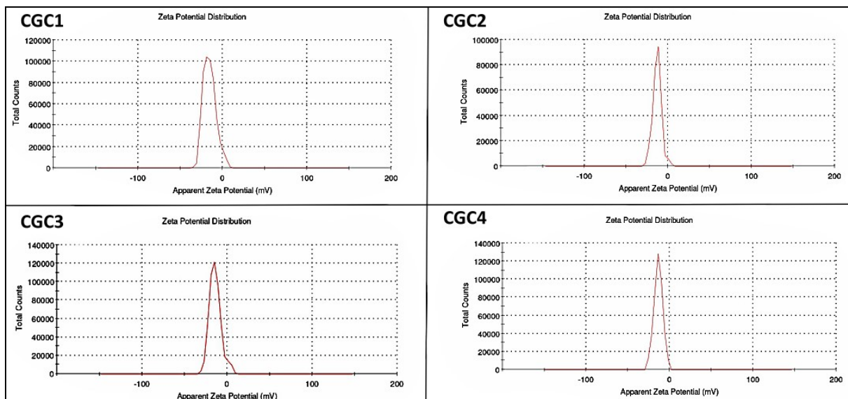
Fig. S2. Zeta potential of pristine and MWCNT, GCN modified \text{CoFe}_2\text{O}_4
