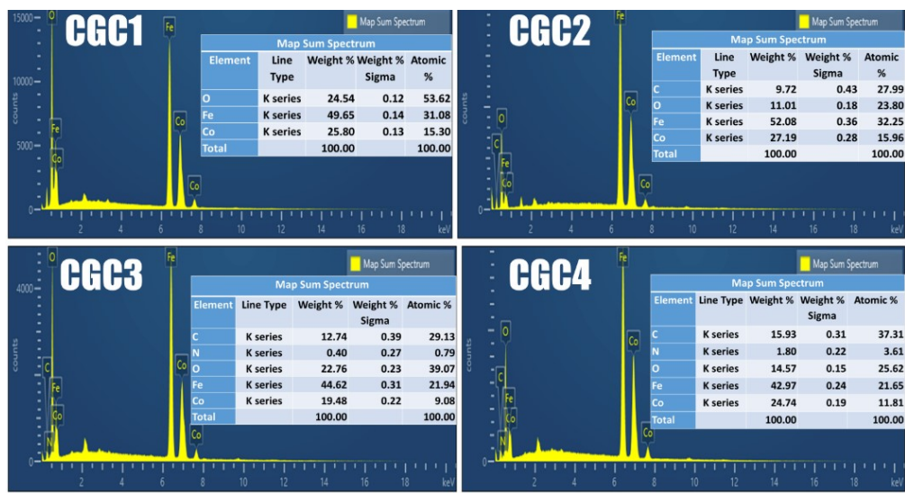
Fig. S1. EDS spectra of CGC1, CGC2, CGC3 and CGC4
