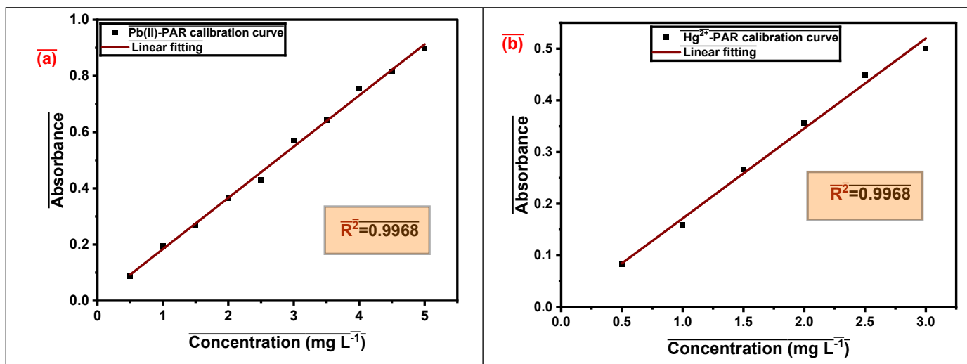
Fig. S1. Calibration curve of (a) Pb 2+ and (b) Hg 2+ with PAR reagent.
