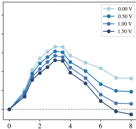
PtGa(100) / RPBE
