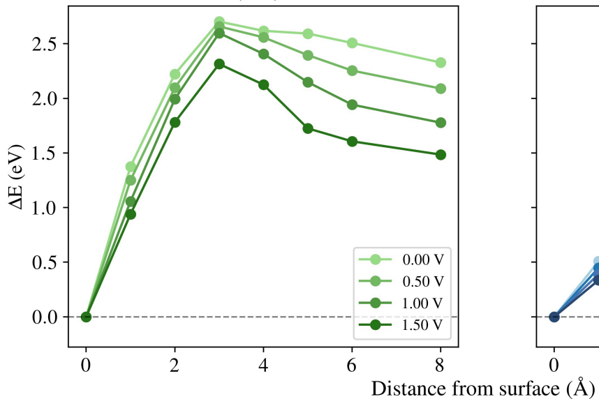
PtGa(100) / PBE
