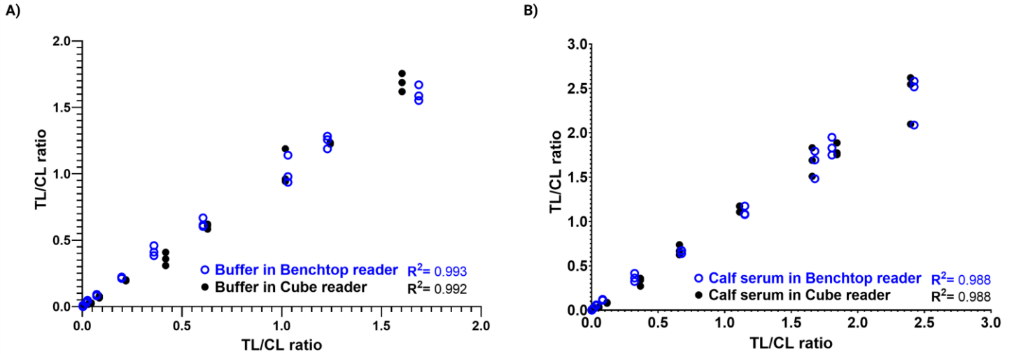
Fig. S1 Comparison of benchtop and portable fluorescence readers. Two linear regression analyses were performed for each serial dilution curve: one with hollow circles, where the X-axis represents the triplicate readings from the benchtop and the y-axis the mean of the data from the portable reader; and another with filled circles, where the X-axis corresponds to the triplicate readings from the portable reader and the Y-axis the mean of the data from the benchtop reader. Data represent serial dilution curves of rLeptin spiked in A) Buffer containing 0.5% BSA and 0.5% Tween-20, and B) 50% Calf serum with final concentrations of 0.25% BSA, 0.5% Tween-20 and 0.5% PEG3350. In both matrices, the TL/CL ratio obtained from both readers follows a linear relationship, with coefficients of determination ( R^2 ) greater than 0.98. R^2 : Coefficient of determination; CL: Control line; LFA: Lateral flow assay; PEG: Polyethylene Glycol; PBS: Phosphate buffered saline; rLeptin: Recombinant leptin; TL: Test line.
