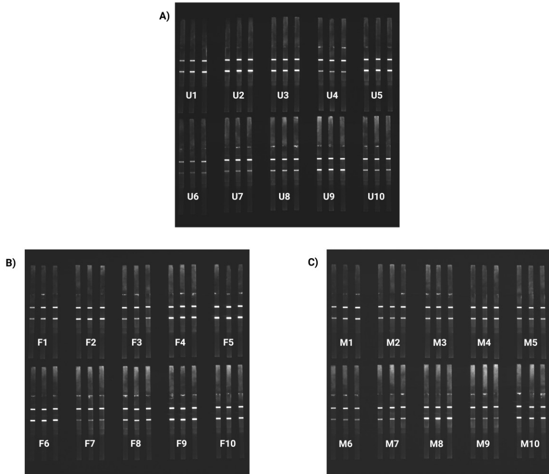
Fig. S3 Images of the 30 human serum samples tested in triplicate at 25% dilution in Running Buffer (0.25% BSA, 0.5% Tween-20, and 0.5% PEG 3350 in 1x PBS) acquired using the FluorChem gel documentation system. The developed LFA successfully detected endogenous leptin in all the samples tested, demonstrating minimal variability. A) Unknown sex samples B) Female samples C) Male samples. BSA: Bovine serum albumin; PEG: Polyethylene Glycol; PBS: Phosphate buffered saline.
