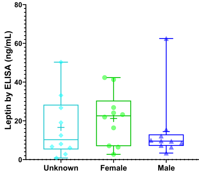
Fig. S2 Leptin levels in human serum samples measured in triplicate using the Human Leptin Quantikine QuickKit ELISA (QK398, R&D Systems). Three groups (n= 10 each) were evaluated: unknown sex, female, and male. The box plots represent, from bottom to top the minimum values, 25th percentile, median, 75th percentile and maximum values. The + symbol indicates the mean.
