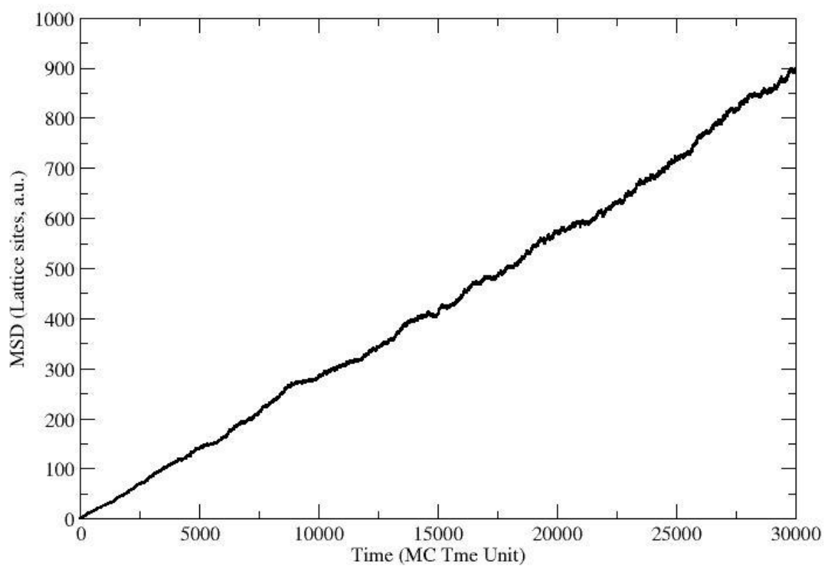
Fig. S1: Mean square displacement of a single protein in a 35DPPC ternary mixture.
