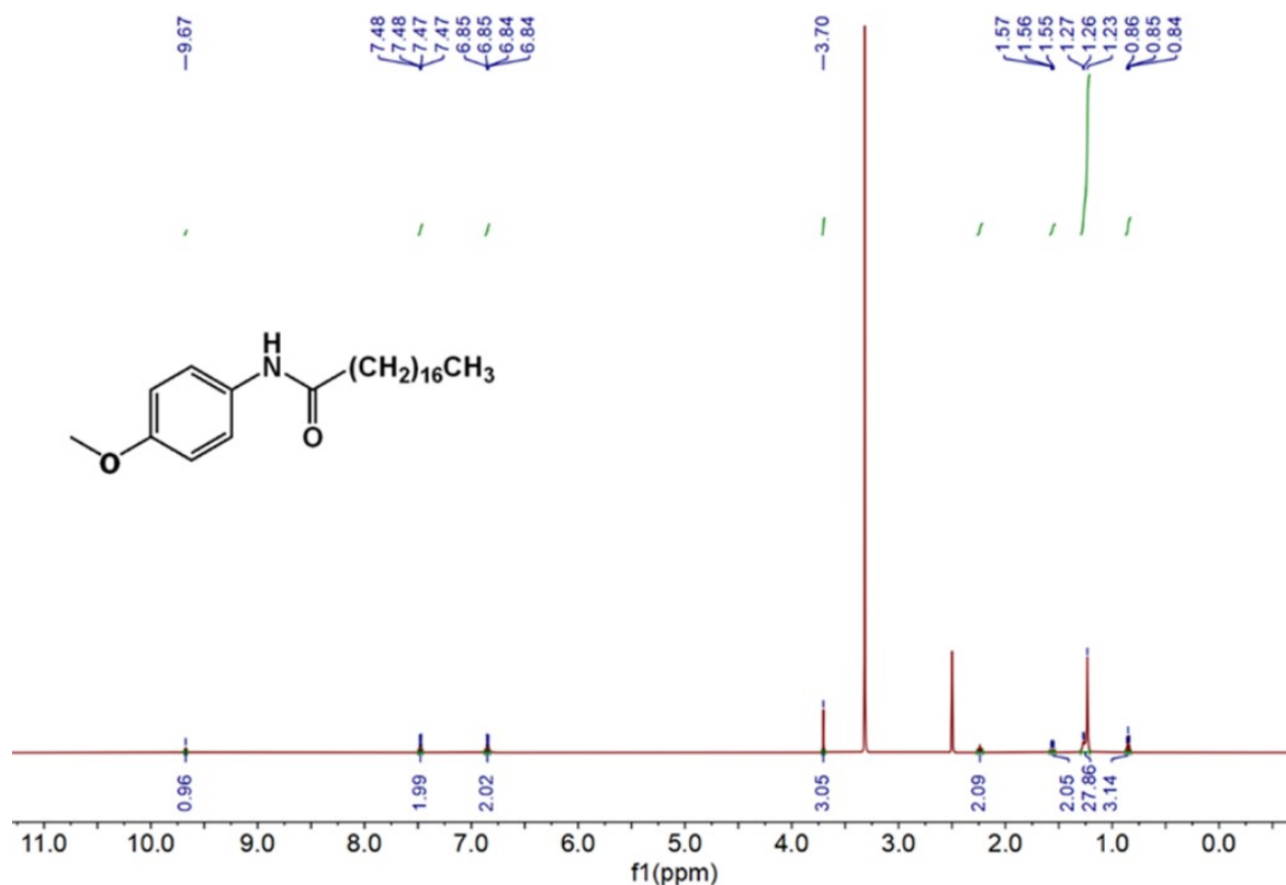
Figure S1. 1 H NMR spectrum of G1 (DMSO-d 6 ).
