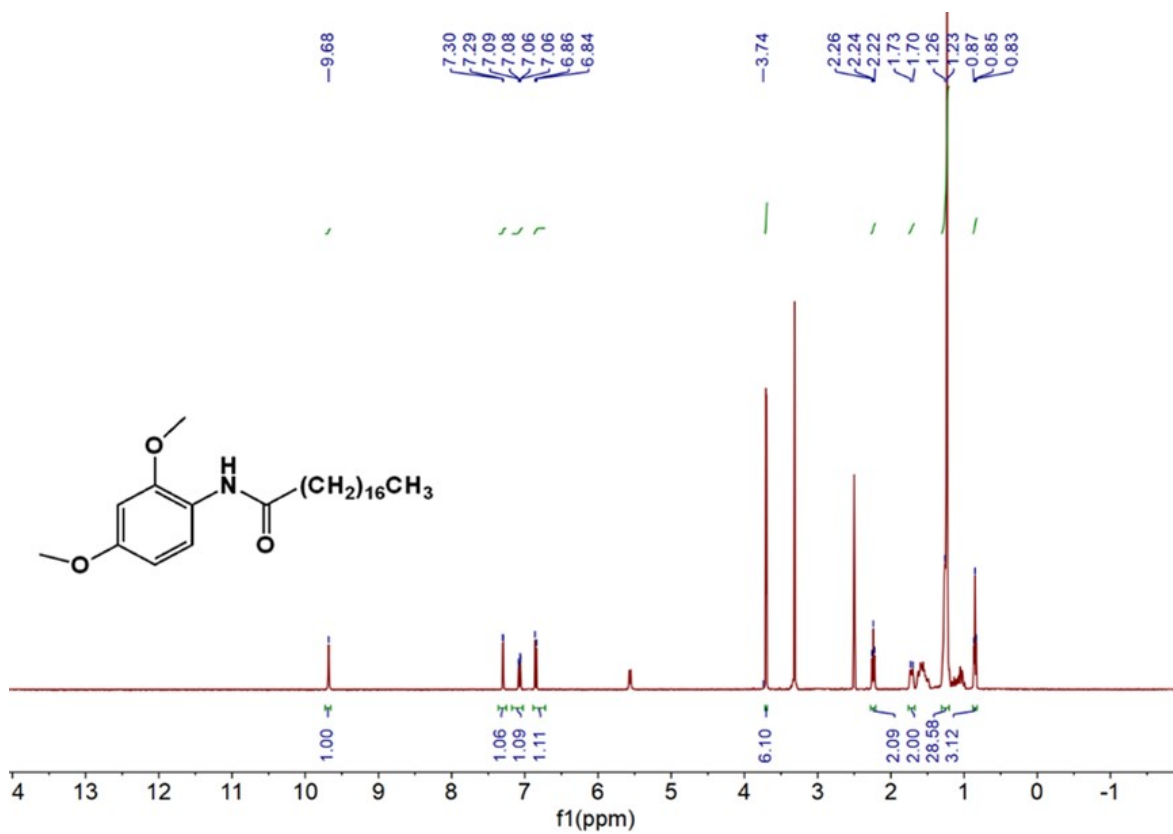
Figure S4. 1 H NMR spectrum of C2 (DMSO-d 6 ).
