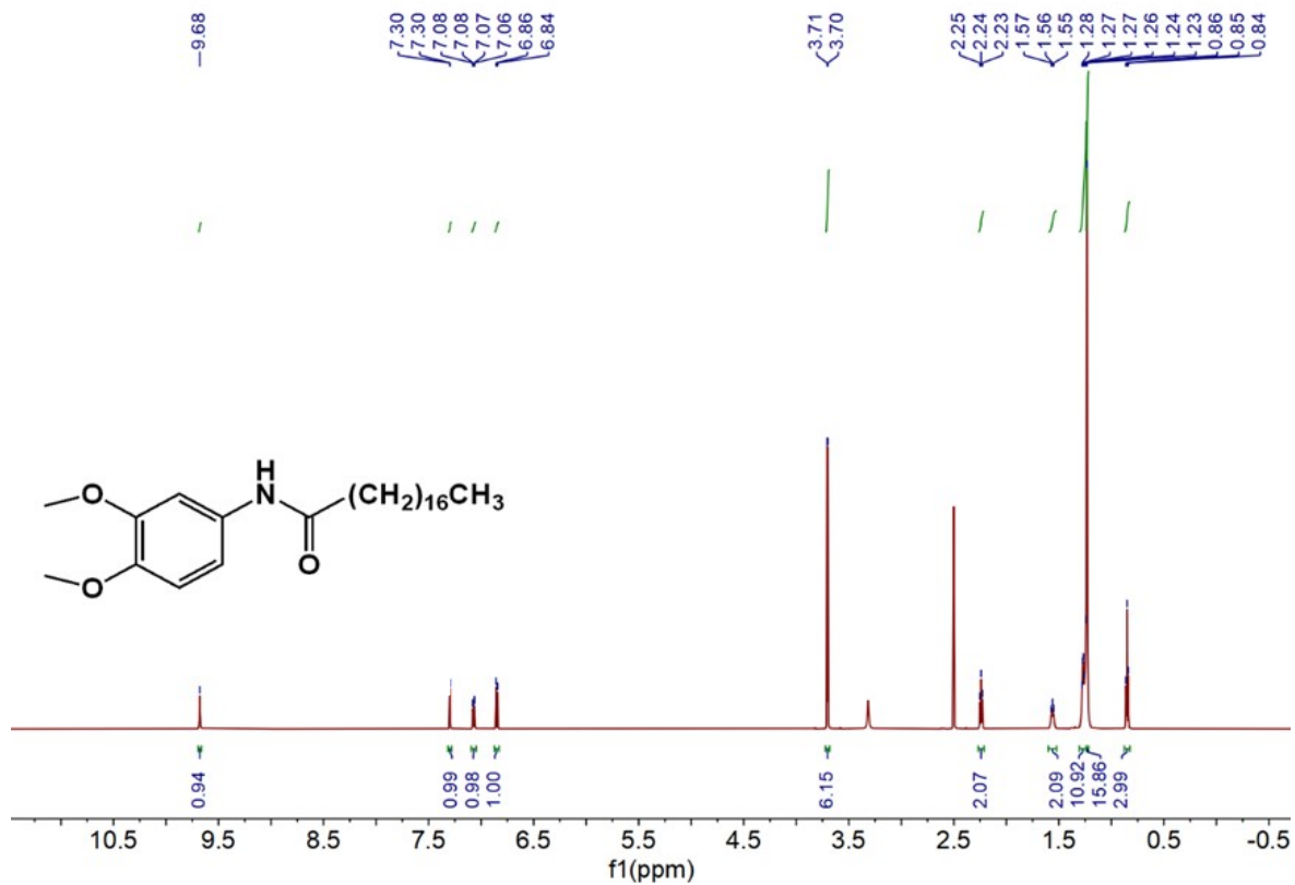
Figure S2. 1 H NMR spectrum of G2.
