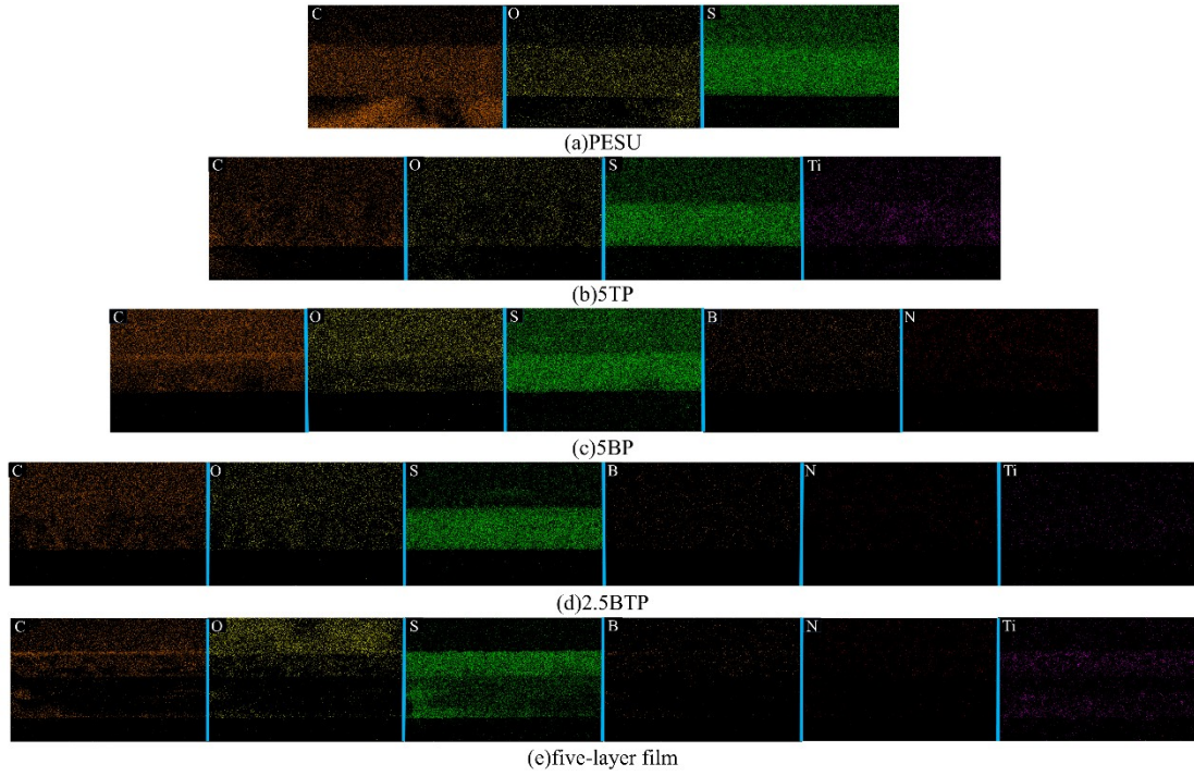
Figure S1. EDS spectra of PESU-based composite films.
