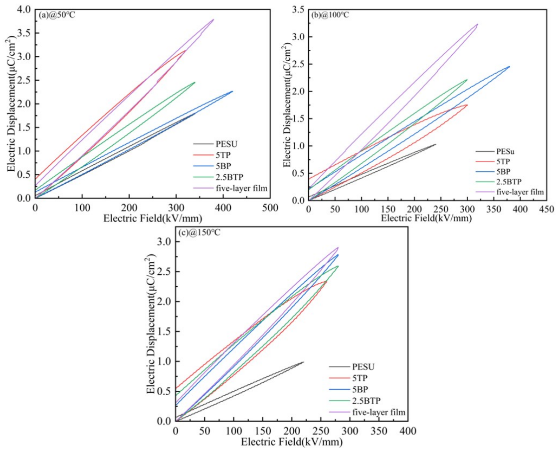
Figure S2. The relationship curve of D-E loops (electric displacement vs. electric field strength) for composites.
