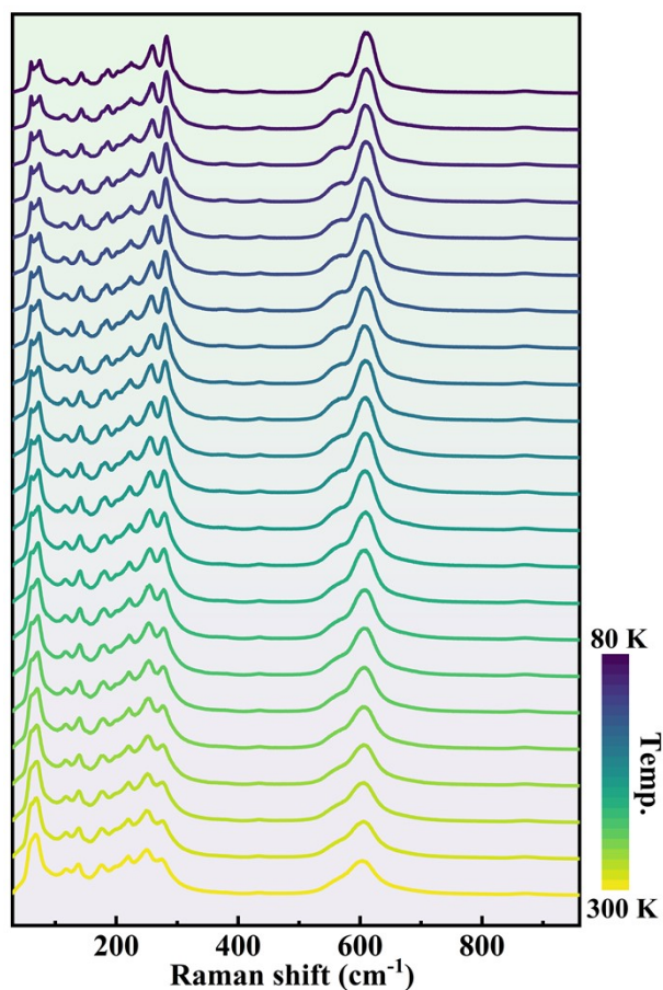
Fig. S1 The in-situ Raman spectra of the NSN-4 sample as a function of temperature. Here, the “Temp.” refers to the measurement temperature.
