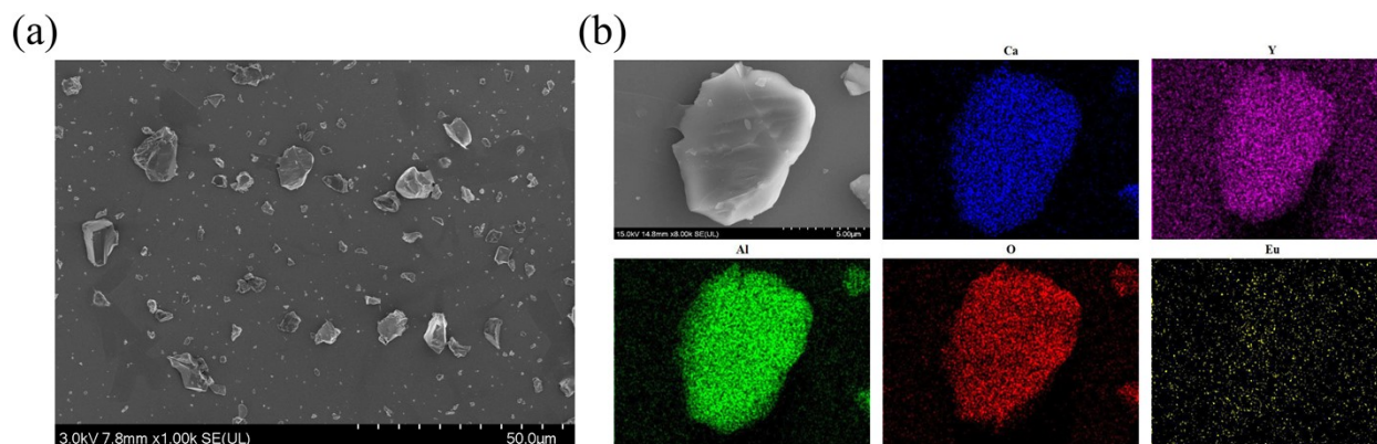
Fig. S1 (a) SEM image of the \text{CaYAl}_3\text{O}_7:0.02\text{Eu} sample (b) EDS spectrum of the \text{CaYAl}_3\text{O}_7:0.02\text{Eu} sample.
