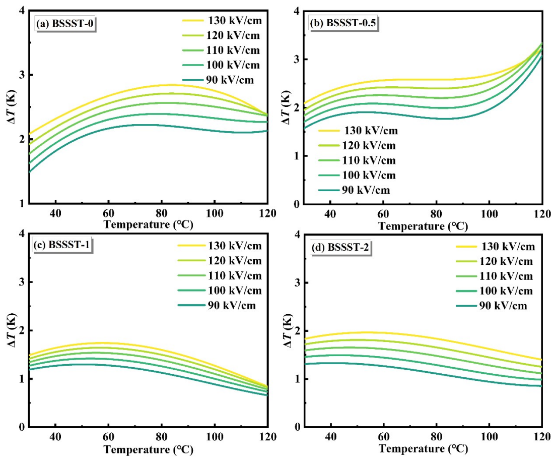
Fig S1. (a-d) Under the same electric field conditions, the relationship graph between \Delta T and temperature for ceramic materials with x values of 0, 0.005, 0.01 and 0.02.
