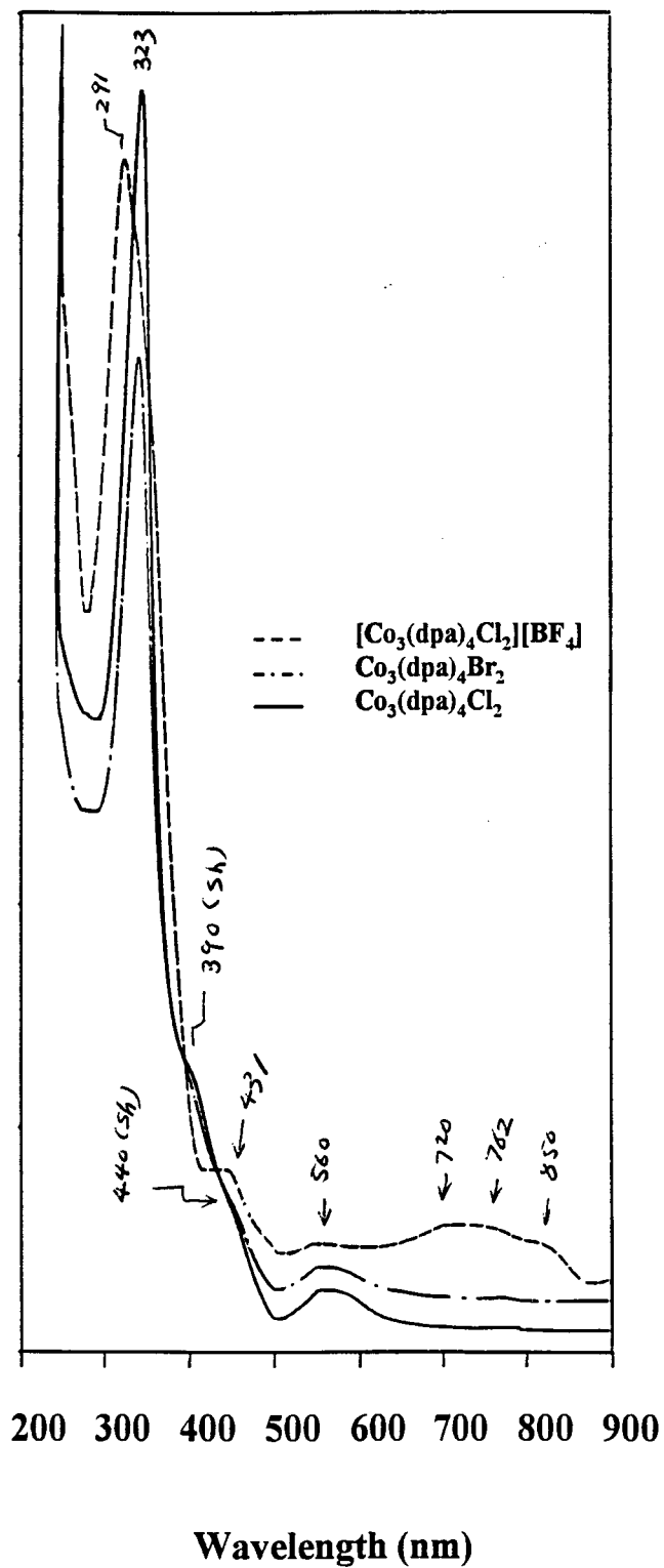
Electronic spectra of \text{CH}_2\text{Cl}_2 solution
