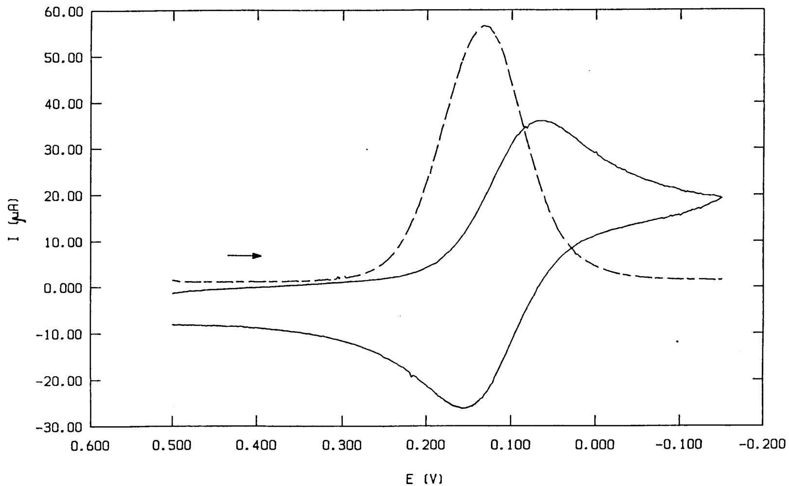
Figure S2. The cyclic (CV) (—) differential pulse (DPV) (-----) voltammograms of 0.001 M complex of [Cu(L1)(H 2 O)Cl]Cl 1a on a Pt sphere electrode in methanol (0.01 M THAP) at 25 °C at 0.05 and 0.001 V s -1 scan rates respectively; pulse height for DPV, 0.05 V.
