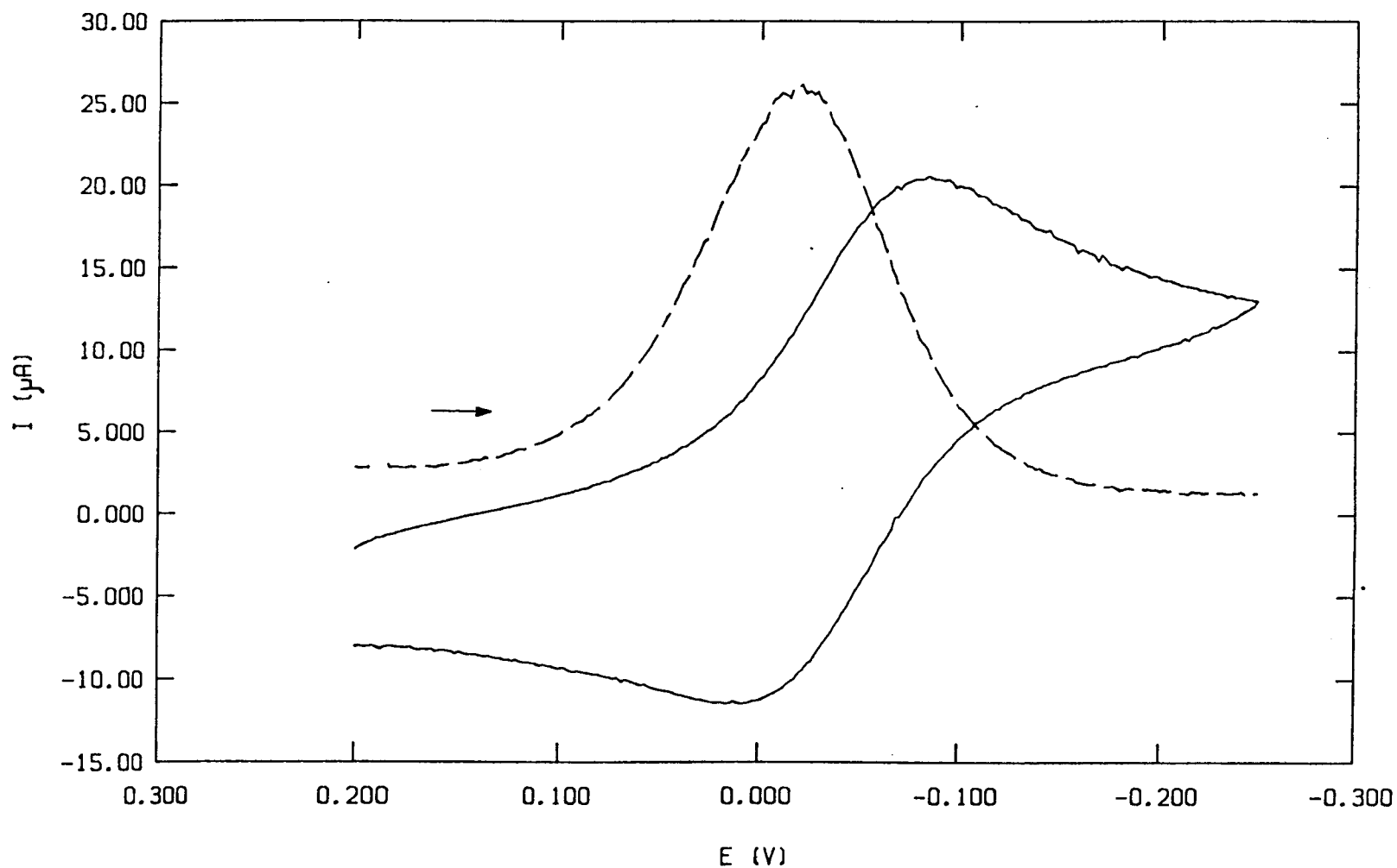
Figure S5. The cyclic (CV) (—) differential pulse (DPV) (-----) voltammograms of 0.001 M complex of [\text{Cu}(\text{L4})](\text{ClO}_4)_2 \cdot 2\text{CH}_3\text{CN} 4 on a Pt sphere electrode in \text{CH}_3\text{CN} (0.01 M TBAP) at 25 °C at 0.05 and 0.001 \text{V s}^{-1} scan rates respectively; pulse height for DPV, 0.05 V.
