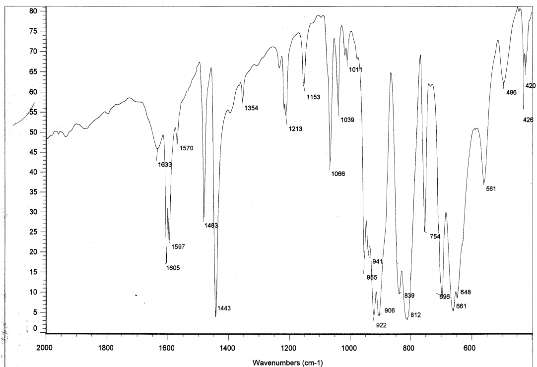
Fig. 2 IR spectra of [\{\text{Cu}(\text{py})_3\}_2\{\text{Cu}(\text{py})_2\}_2(\alpha\text{-Mo}_8\text{O}_{26})] (2)
