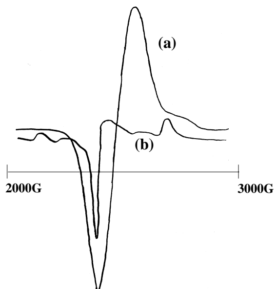
Fig. 1 ESR spectra of 1 (a) and 3 (b).
