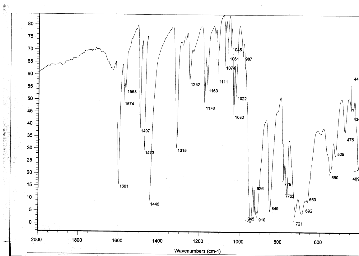
Fig. 1 IR spectra of [\{\text{Cu}(2,2'\text{-bipy})_2\}_2(\beta\text{-Mo}_8\text{O}_{26})] ( 1 )
