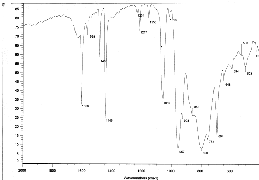
Fig. 3 IR spectra of [\text{Cu}(\text{py})_2]_4[(\text{SO}_4)\text{Mo}_{12}\text{O}_{36}] (3)
