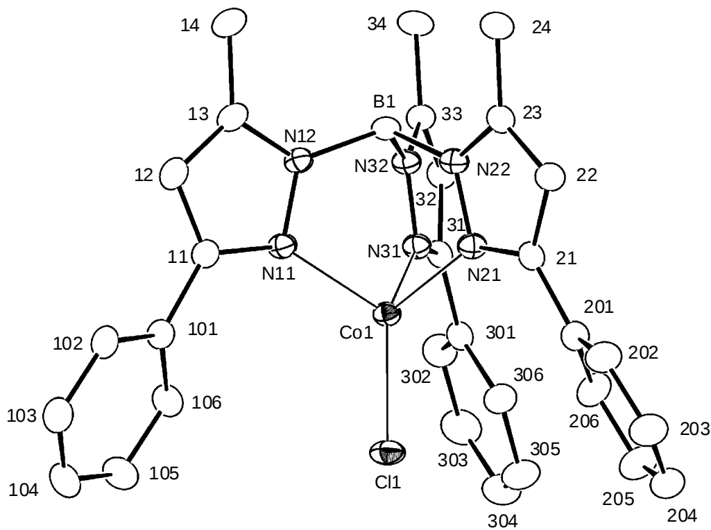
Figure S4. Atomic numbering schemes for 2 Co .
