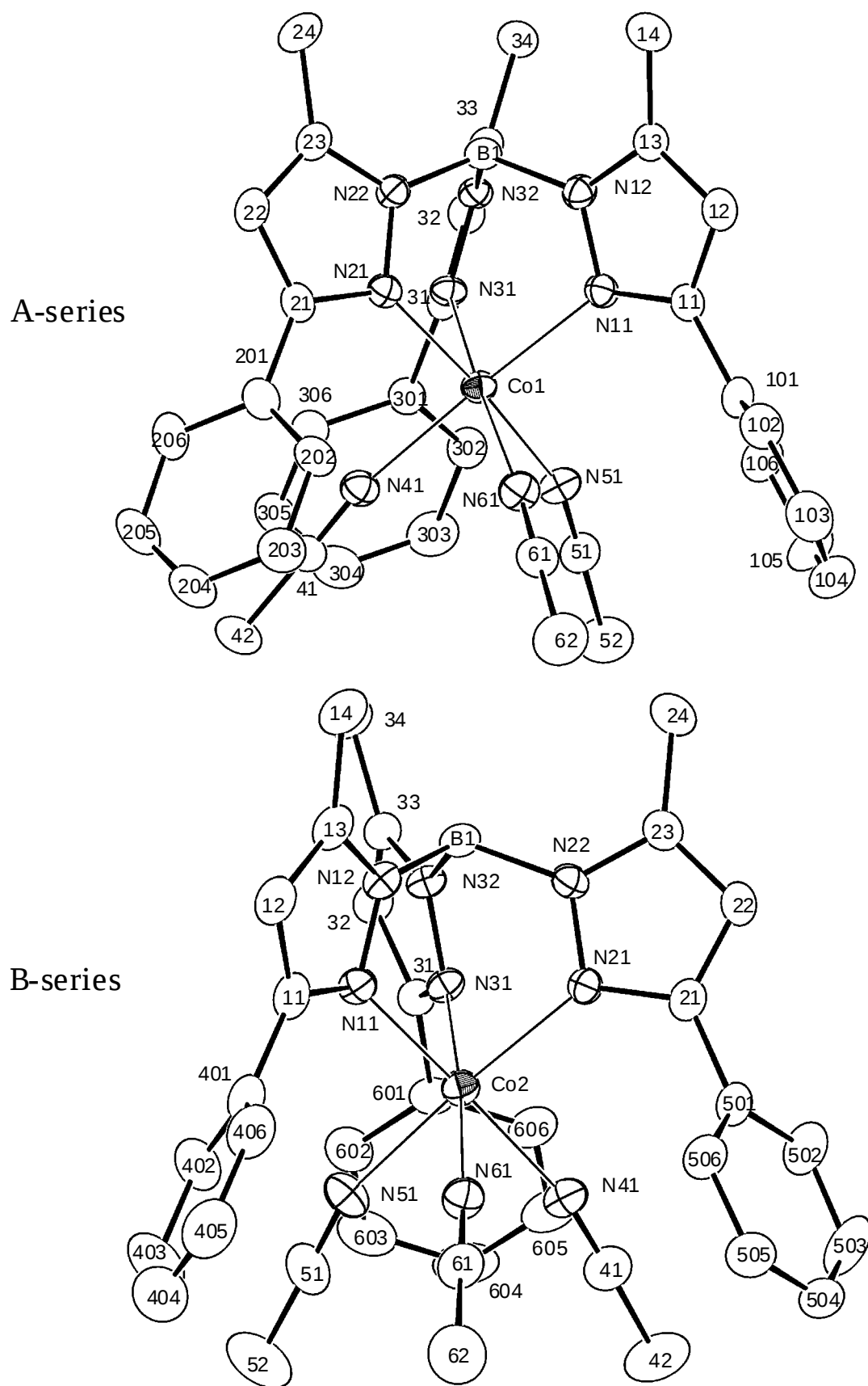
Figure S2. Atomic numbering schemes for the cationic parts of 1Co .
