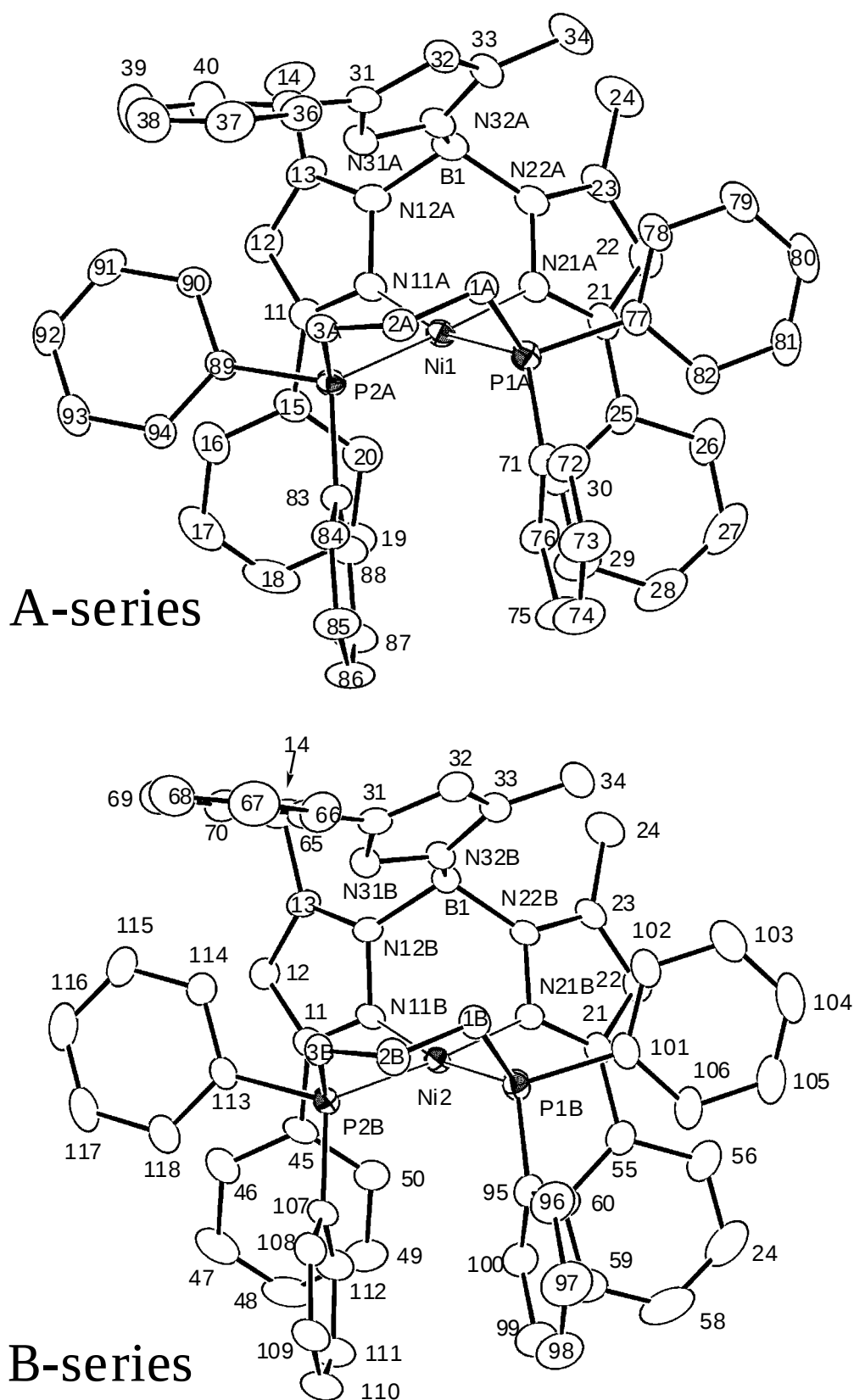
Figure S13. Atomic numbering schemes for the cationic parts of 14b .
