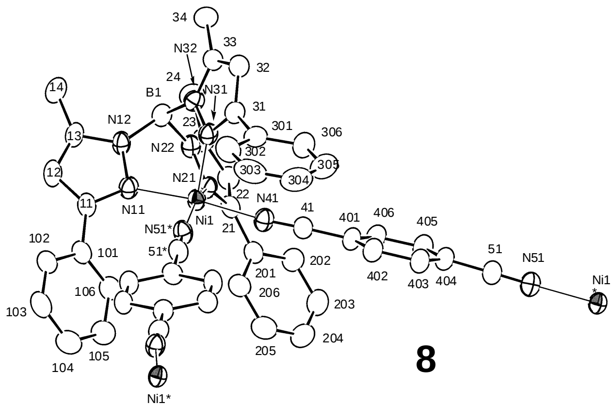
Figure S8. Atomic numbering schemes for the cationic parts of 7 and 8 .
