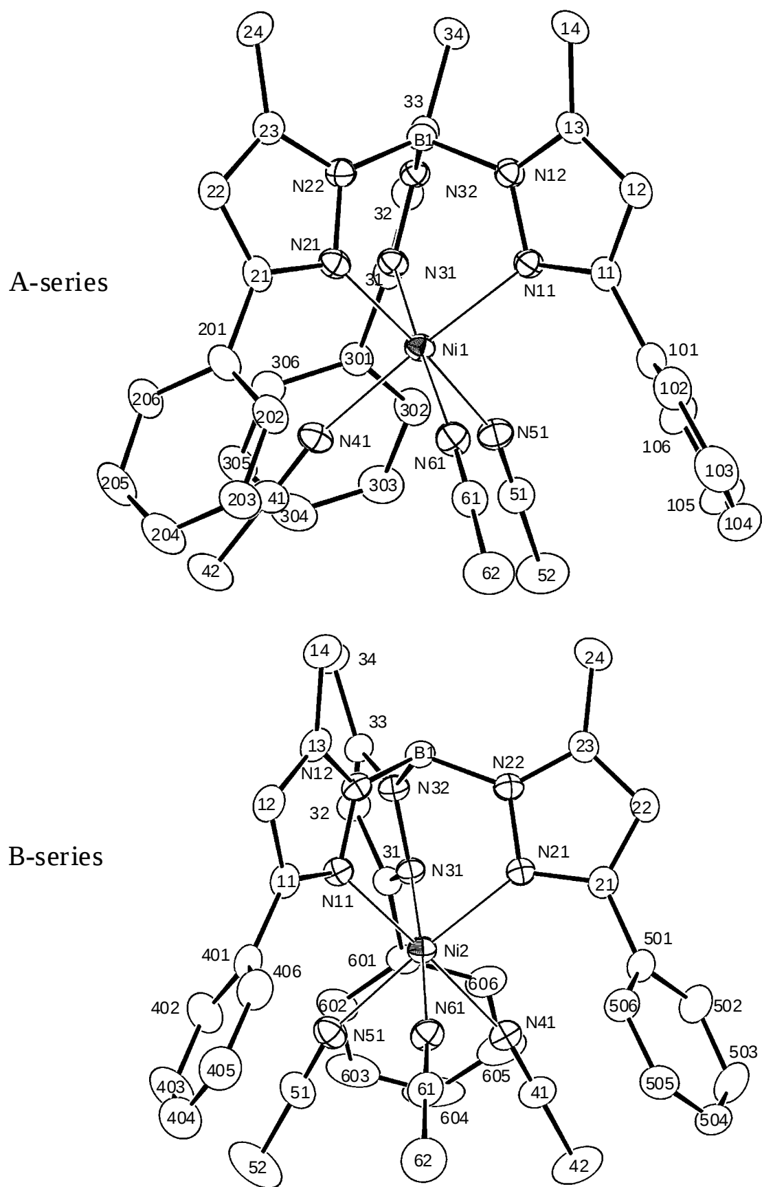
Figure S1. Atomic numbering schemes for the cationic parts of 1Ni .
