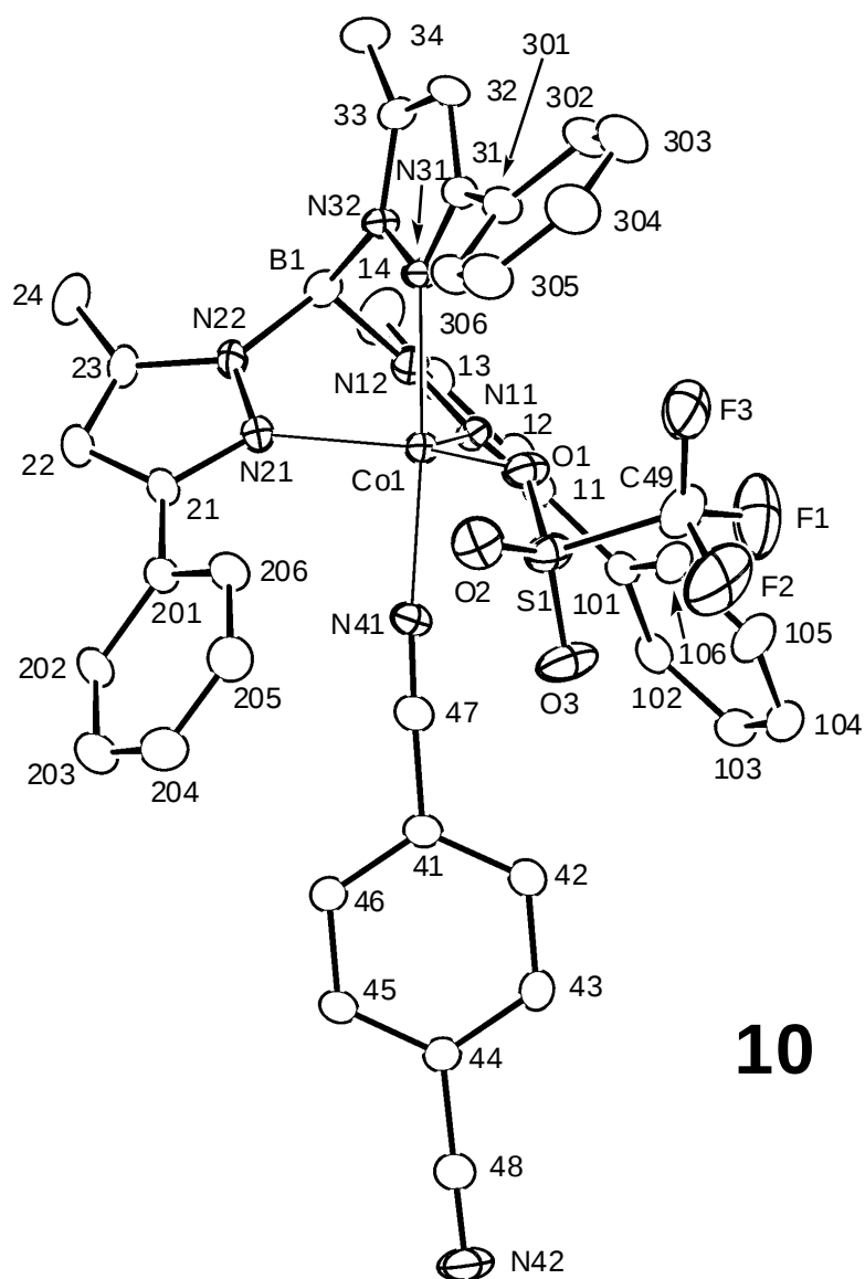
Figure S9. Atomic numbering schemes for 9 and 10 .
