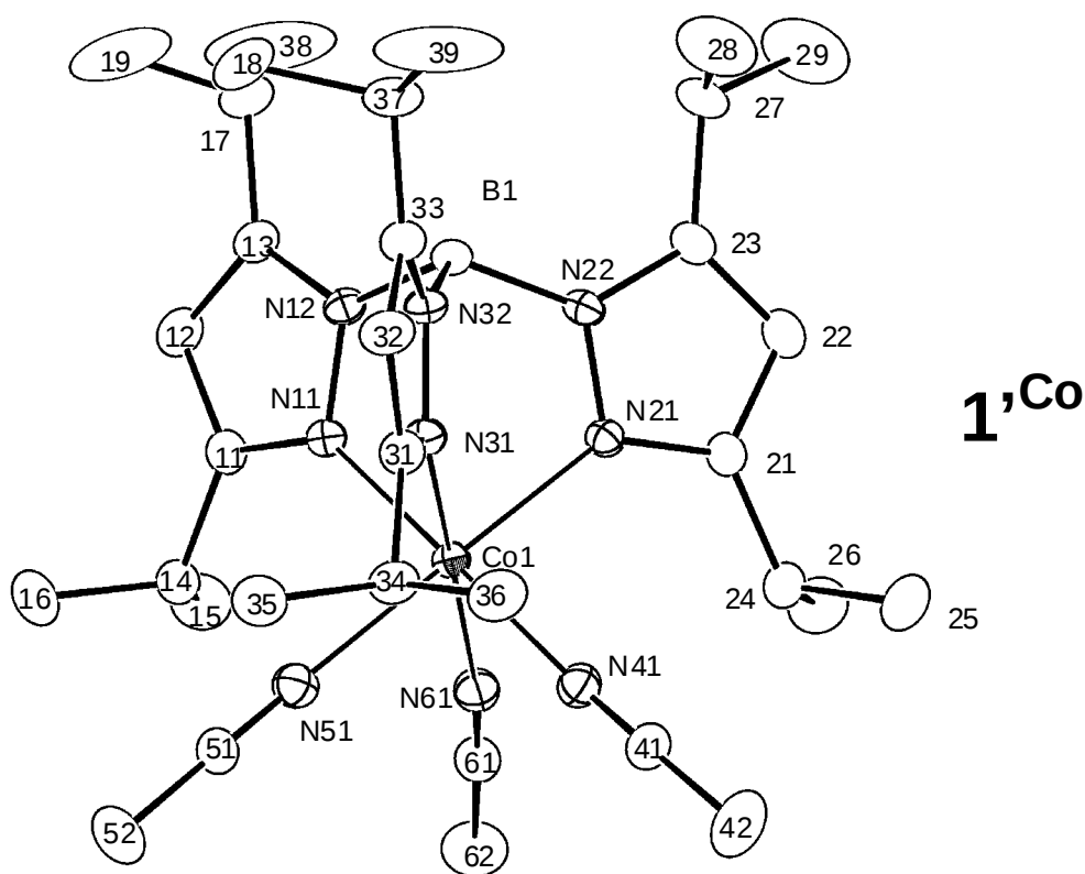
Figure S3. Atomic numbering schemes for the cationic parts of 1' .
