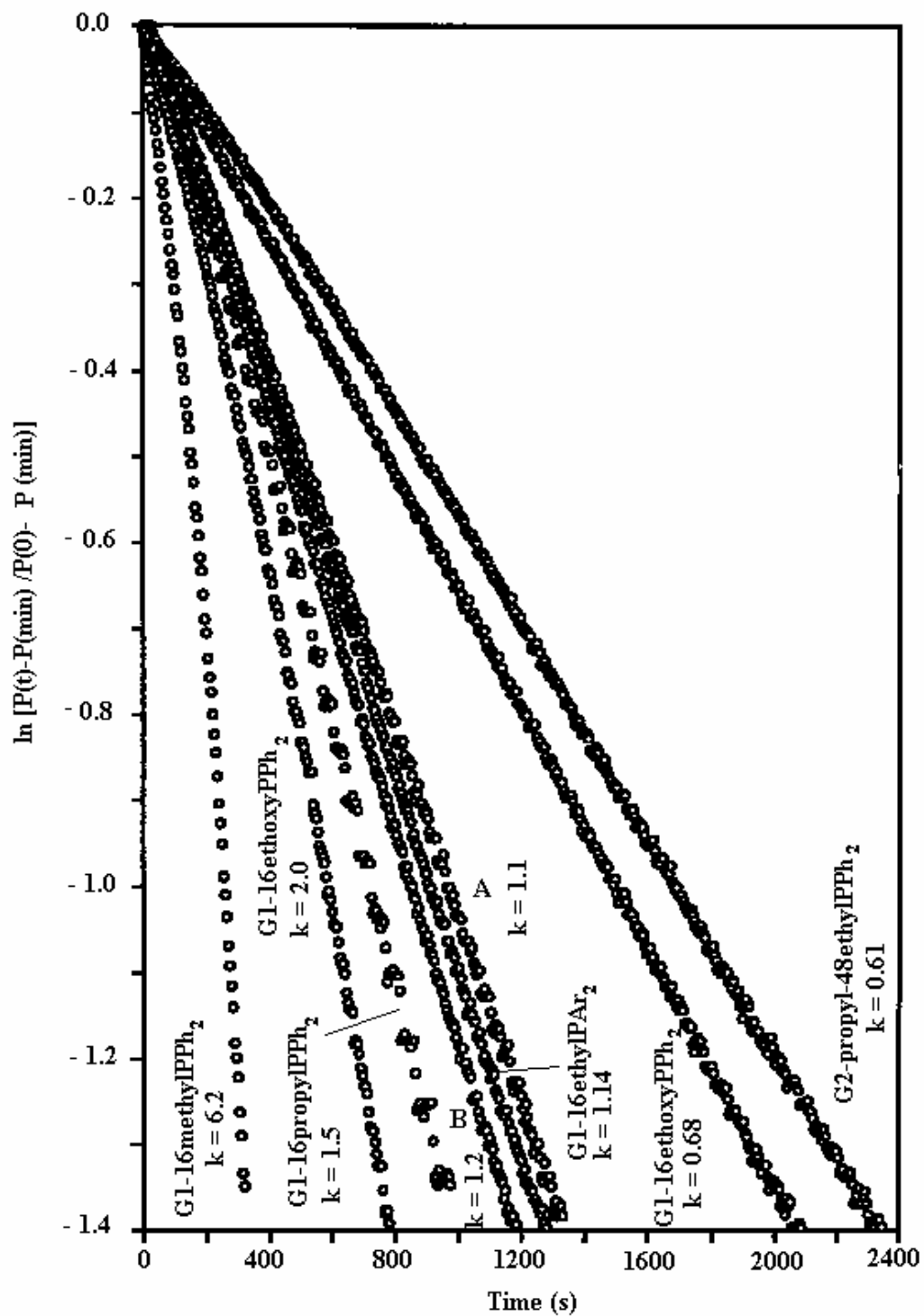
Fig. S2 Effect of the dendrimer structure on the rate of hydroformylation of oct-1-ene ( k in 10^{-3} \text{ s}^{-1} ) ( [\text{Rh}] = 3.77 \times 10^{-3} \text{ mol} \cdot \text{dm}^{-3} , P/\text{Rh} = 5.4/1 , \text{H}_2/\text{CO} 10 bar, 120^\circ\text{C} ).
