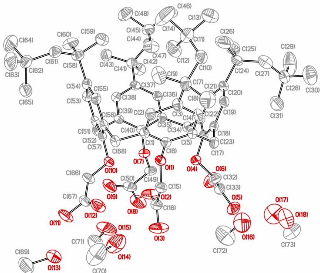
Atom numbering scheme for compound 1.
