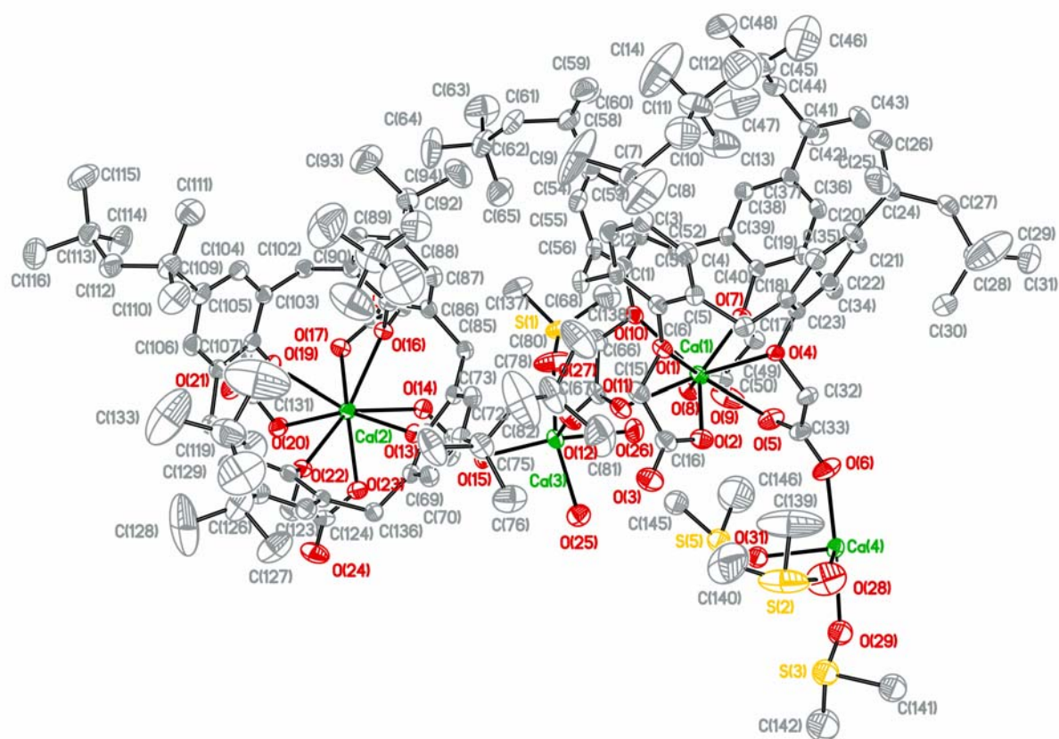
Atom numbering scheme for compound 2. (Lattice solvent molecules not included)
