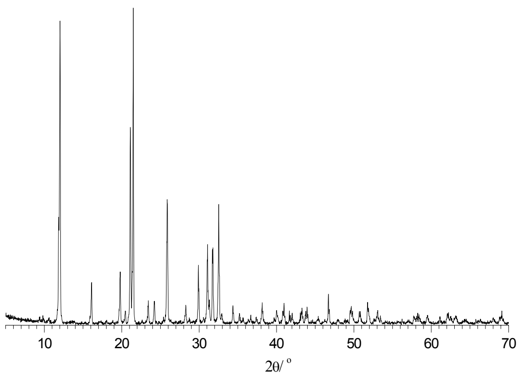
Powder X-ray diffraction pattern of as-synthesized zinc phosphate
