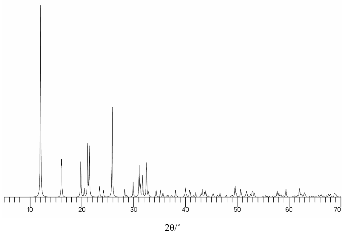
Simulated powder X-ray diffraction pattern based on the single crystal solution
