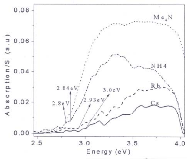
Optical absorption spectra of AGa 3 (A= Cs, Rb, NH 4 and Me 4 N) compounds
