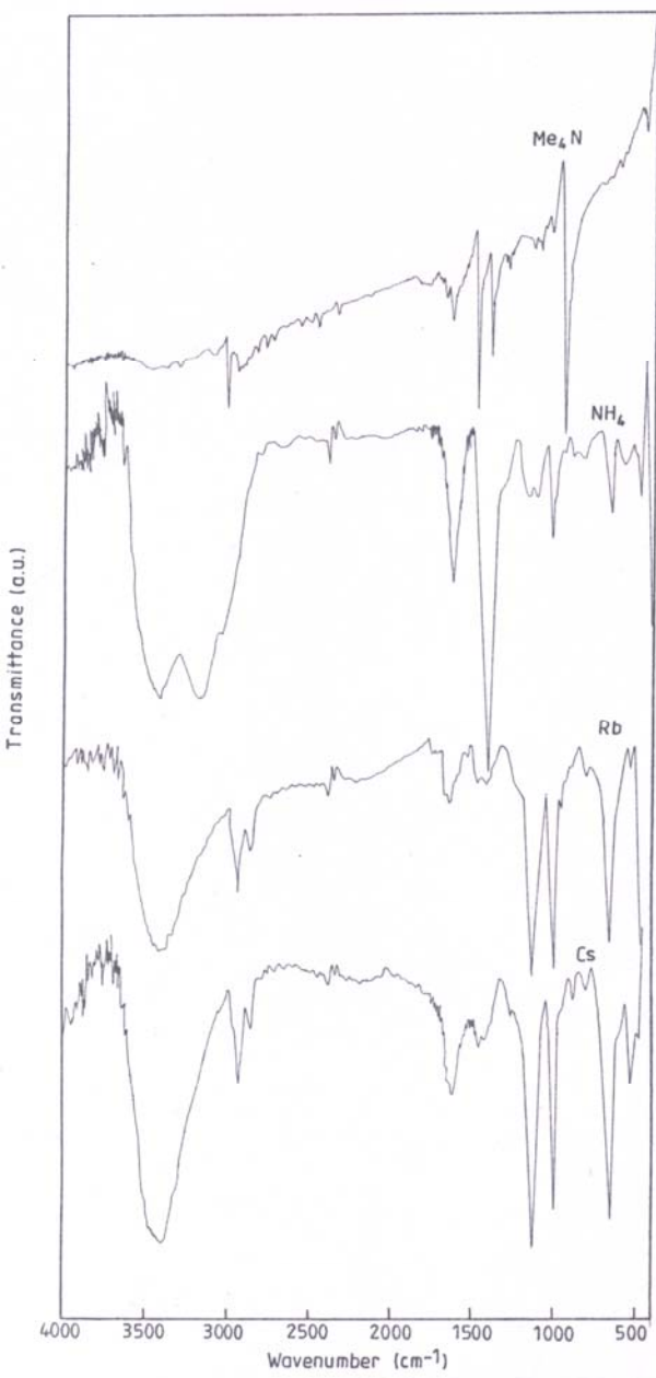
IR spectra of \text{AGaS}_3 (A= Cs, Rb, \text{NH}_4 and \text{Me}_4\text{N} ) compounds
