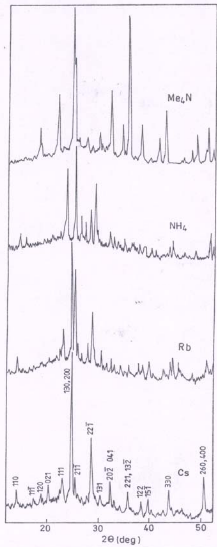
Powder XRD patterns of \text{AGaS}_3 ( A = \text{Cs}, \text{Rb}, \text{NH}_4 and \text{Me}_4\text{N} ) compounds.
