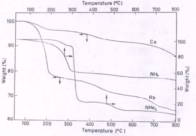
Thermogravimetric curves of AGaS_3 (A = Cs, Rb, NH_4 and Me_4N ) compounds.
