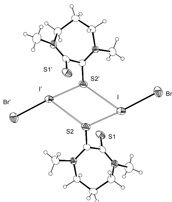
Fig. S1. Molecular drawing of the dimeric species [1 \cdot IBr]_2 . The prime denotes the symmetry operator: -x + 1, -y, -z + 1 .
