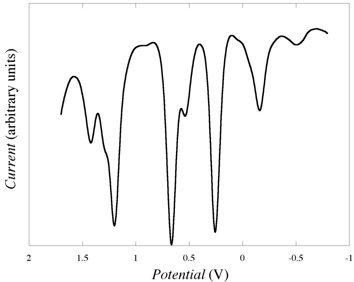
Figure S2. Differential pulse voltammogram of 1 performed in 0.1 M [n\text{-Bu}_4\text{N}][\text{PF}_6] in \text{CH}_2\text{Cl}_2 versus standard Ag/AgCl reference electrode.
