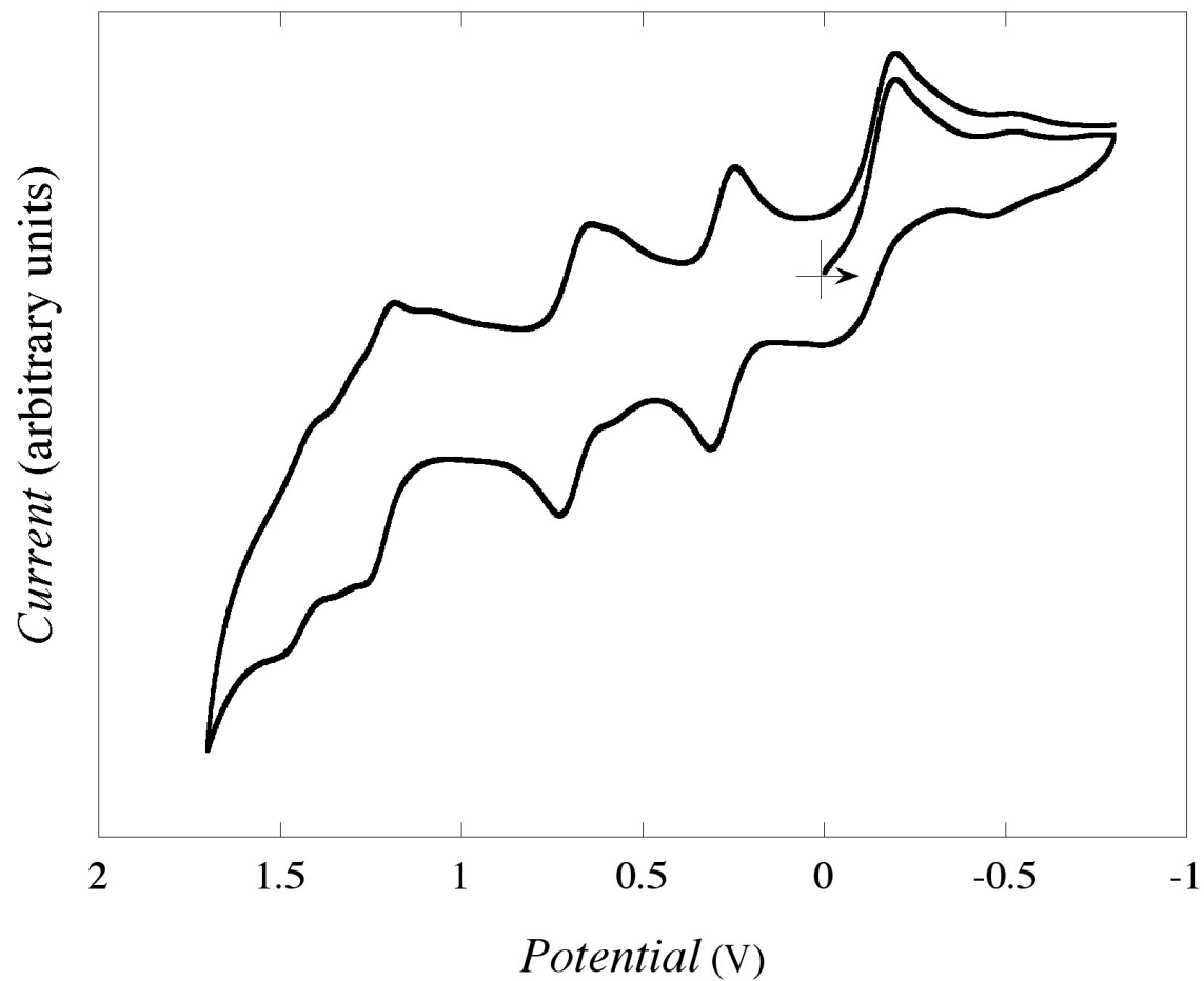
Figure S1. Cyclic voltammogram of 1 performed in 0.1 M [ n -Bu 4 N][PF 6 ] in CH 2 Cl 2 versus standard Ag/AgCl reference electrode.
