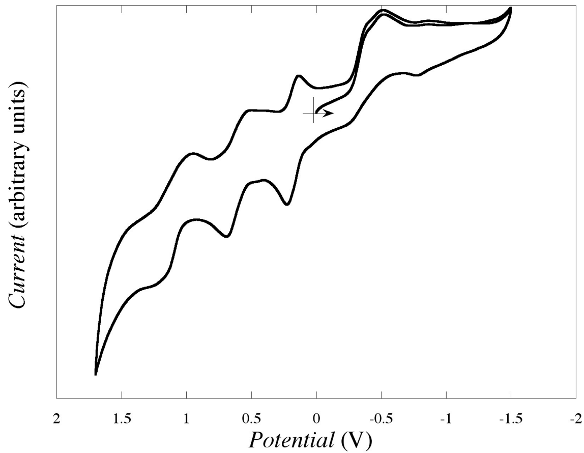
Figure S3. Cyclic voltammogram of 2 performed in 0.1 M [ n -Bu 4 N][PF 6 ] in CH 2 Cl 2 versus standard Ag/AgCl reference electrode.
