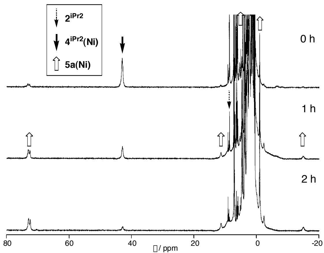
Figure 4. ^1\text{H-NMR} spectral change of a mixture of 2^{\text{iPr}_2} and 4^{\text{iPr}_2(\text{Ni})} at -20^\circ\text{C} . observed at 400 MHz.
