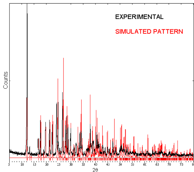
Figure S2 The simulated (red) and experimental (black) powder patterns of [\text{Ag}_2(\text{dpzpy})(\text{NO}_3)_2]_\infty 2 .
