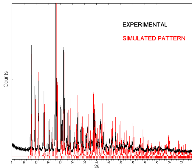
Figure S1 The simulated (red) and experimental (black) powder patterns of [\text{Ag}_2(\text{dpztz})(\text{NO}_3)_2]_\infty 1 .
