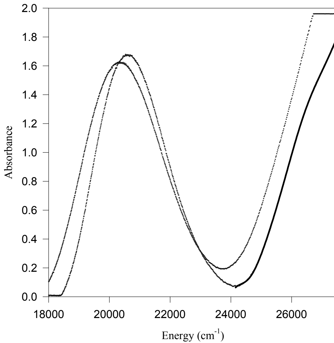
Fig. S1(a) Nafion film UV-visible absorption spectrum of [\text{Co}(\text{PrN}_4\text{S}_2\text{amp})]^{3+} at room temperature and 14 K - spin allowed transitions
