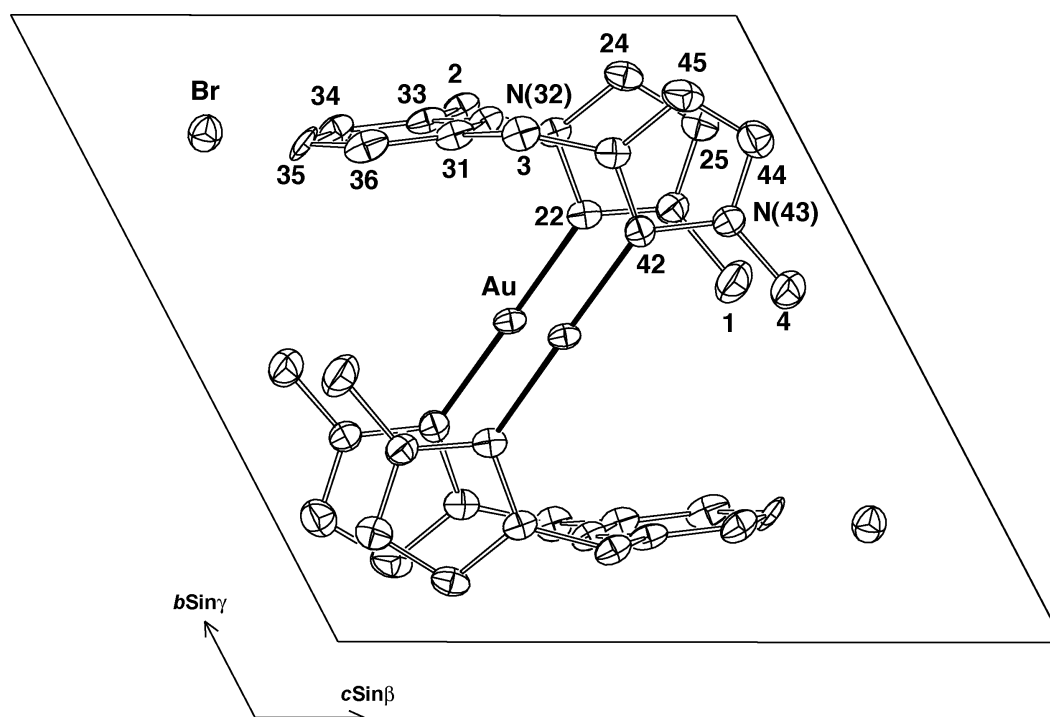
Fig. S2 Unit cell contents of 9 , projected down a .
