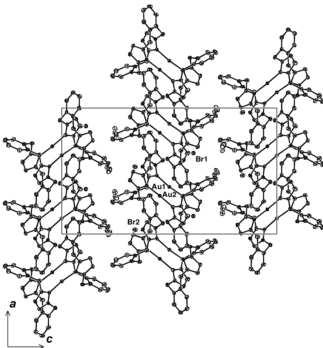
Fig. S1 (a) Unit cell contents of 3 projected down b , showing the layering of the structure.
