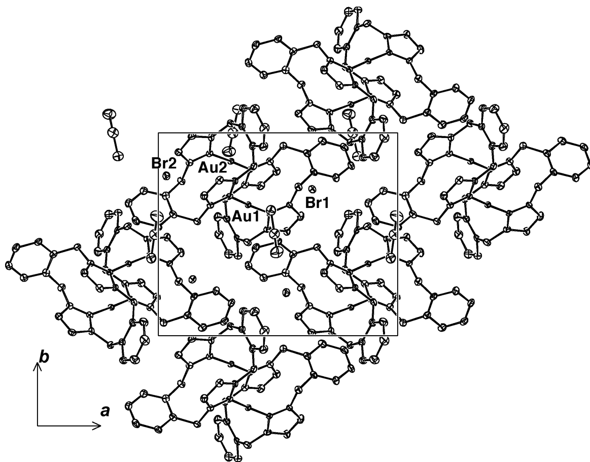
Fig. S1 (b) A single layer of 3 projected down c .
