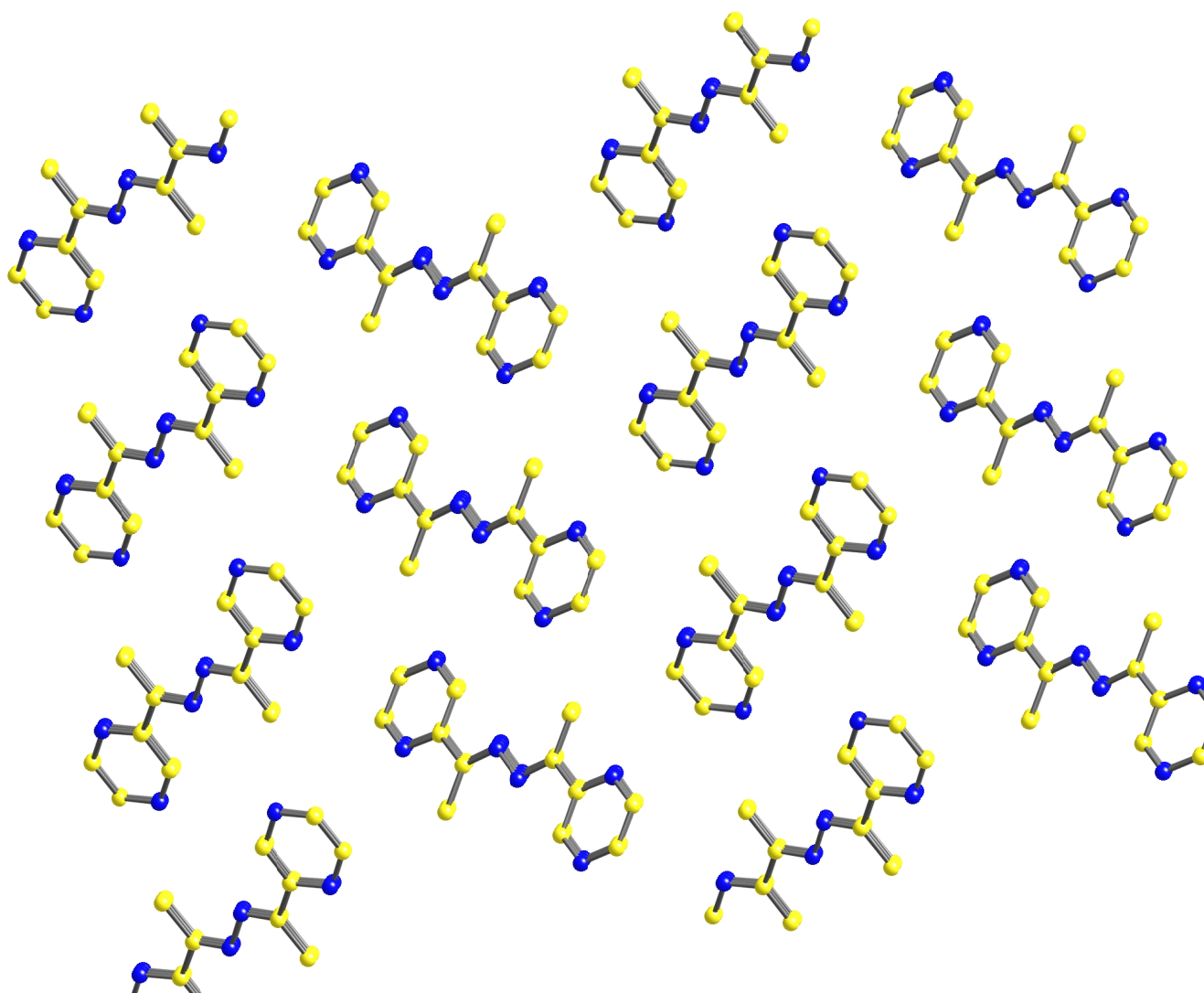
Figure S1: View showing the herringbone style packing of the \pi -stacked columns in the structure of ligand L_a
