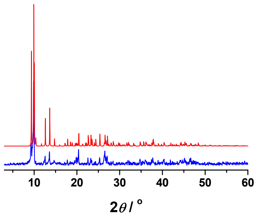
Figure S1 Simulated and experimental XRPD data of 2 .
