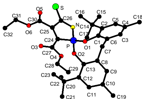
Fig. 3. A drawing of 3.C_6H_5CH_3 showing only the non-hydrogen atoms; solvent atoms are not shown. Only selected atoms labelled.
