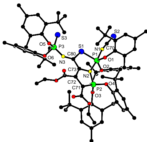
Fig. 4. Molecular structure of 5.2CH_2Cl_2 ; solvent and hydrogen atoms are omitted. Only selected atoms are labelled.
