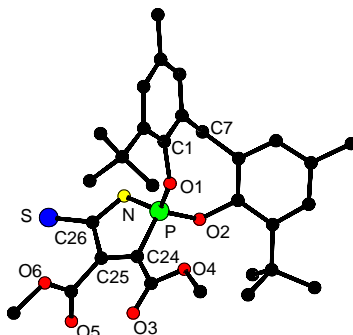
Fig. 2. Molecular structure of 2 showing all non-hydrogen atoms. Only selected atoms labelled.
