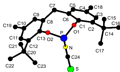
Fig. 1. Molecular structure of 1 showing all non-hydrogen atoms.
