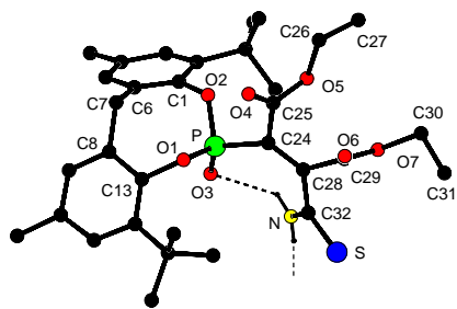
Fig. 5. A drawing showing the molecular structure of 8 . All hydrogen atoms except those on nitrogen are omitted for clarity.
