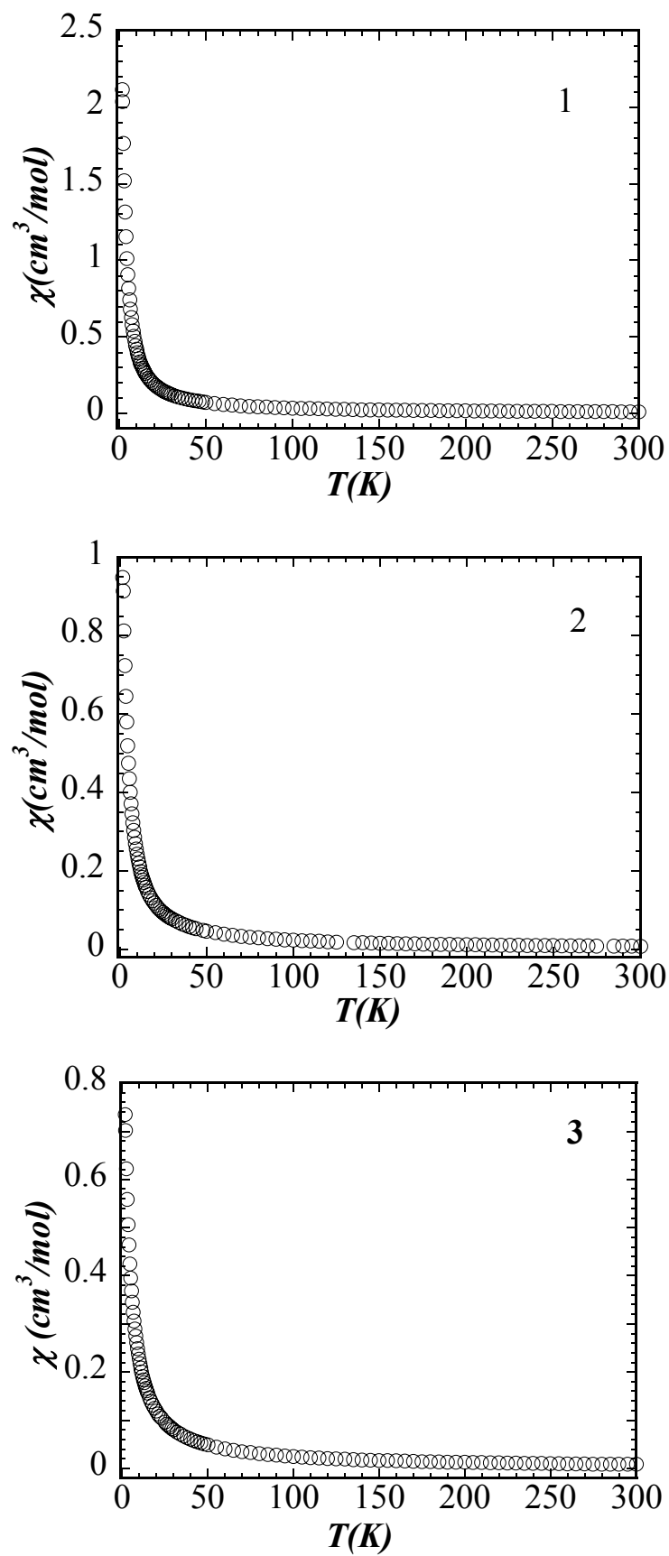
Fig. S2 Temperature dependence of susceptibility for 1 , 2 and 3 . The susceptibility given is per three
