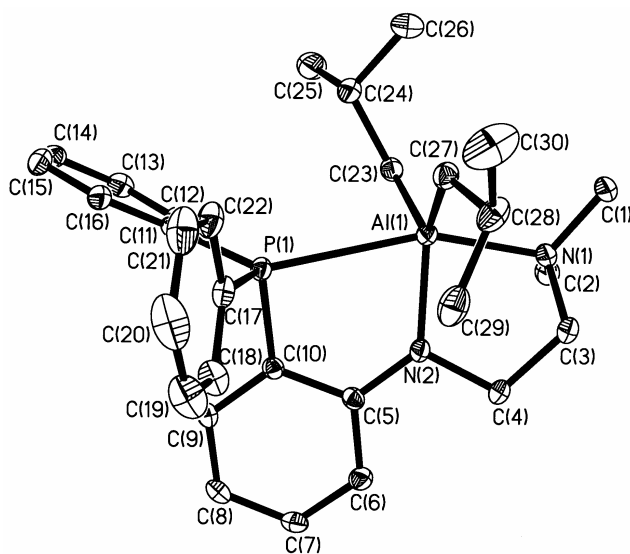
Figure S2. Molecular structure of [PNN]Al( i -Bu) 2 with thermal ellipsoids drawn at the 35% probability level.
