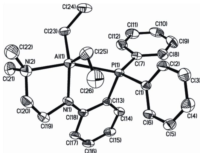
Figure S1. Molecular structure of [PNN]AlEt 2 with thermal ellipsoids drawn at the 35% probability level.
