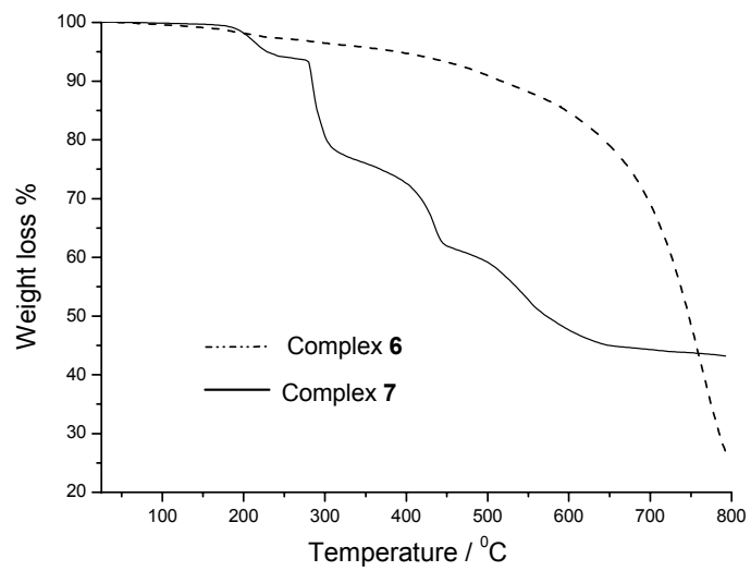
Figure S1. TGA plot of 6 and 7 .
