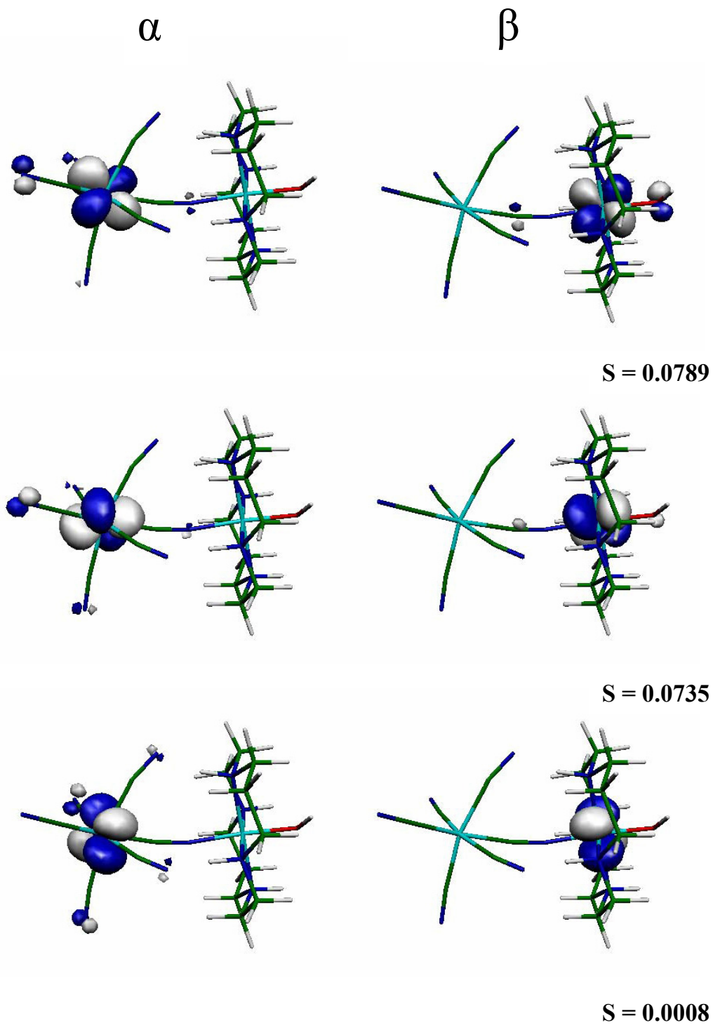
Figure 6. Magnetic orbitals for compounds 1 at the BS-B3LYP level of theory, as obtained from the corresponding orbital transformation (see text).
