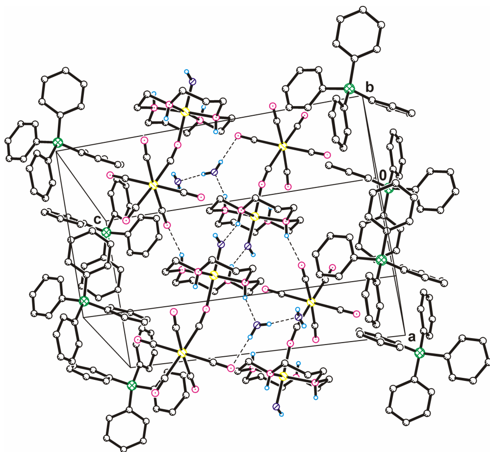
Figure 3 – Packing structure of the crystal 1 , showing its layered structure and the H-bonding.
